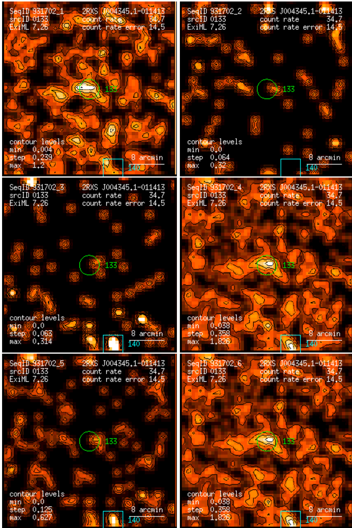
Figure 133: RASS 931702: detection 0133: band rate images, Gaussian filter: (1) PSPC channels 11 – 41, (2) 52 – 90, (3) 91 – 201, (4) 11 – 235, (5) 52 – 201, (6) 11 – 201. Broad band rates in counts/ks. Band rate contour levels in counts/ks/arcmin 2 .
