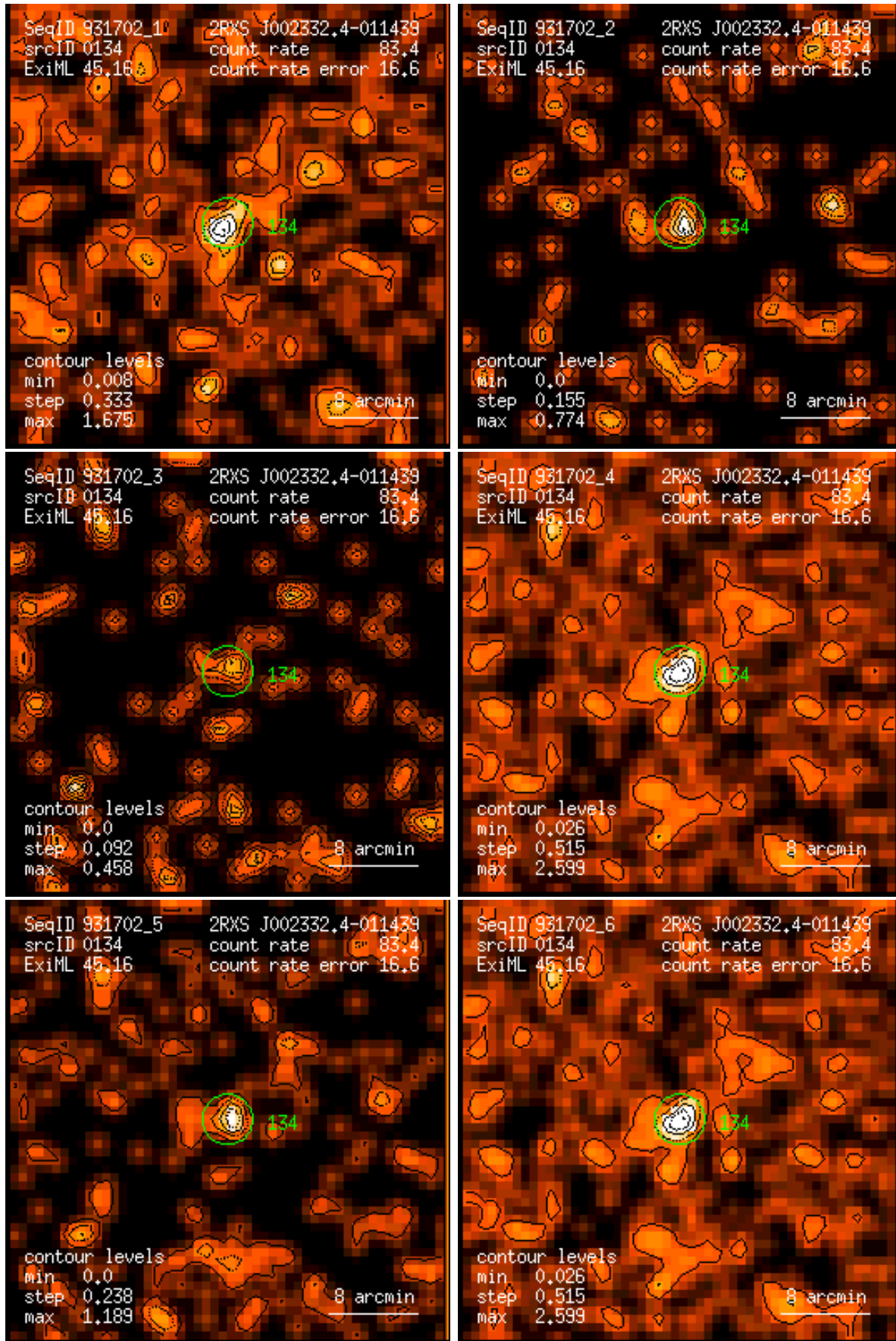
Figure 134: RASS 931702: detection 0134: band rate images, Gaussian filter: (1) PSPC channels 11 – 41, (2) 52 – 90, (3) 91 – 201, (4) 11 – 235, (5) 52 – 201, (6) 11 – 201. Broad band rates in counts/ks. Band rate contour levels in counts/ks/arcmin 2 .
