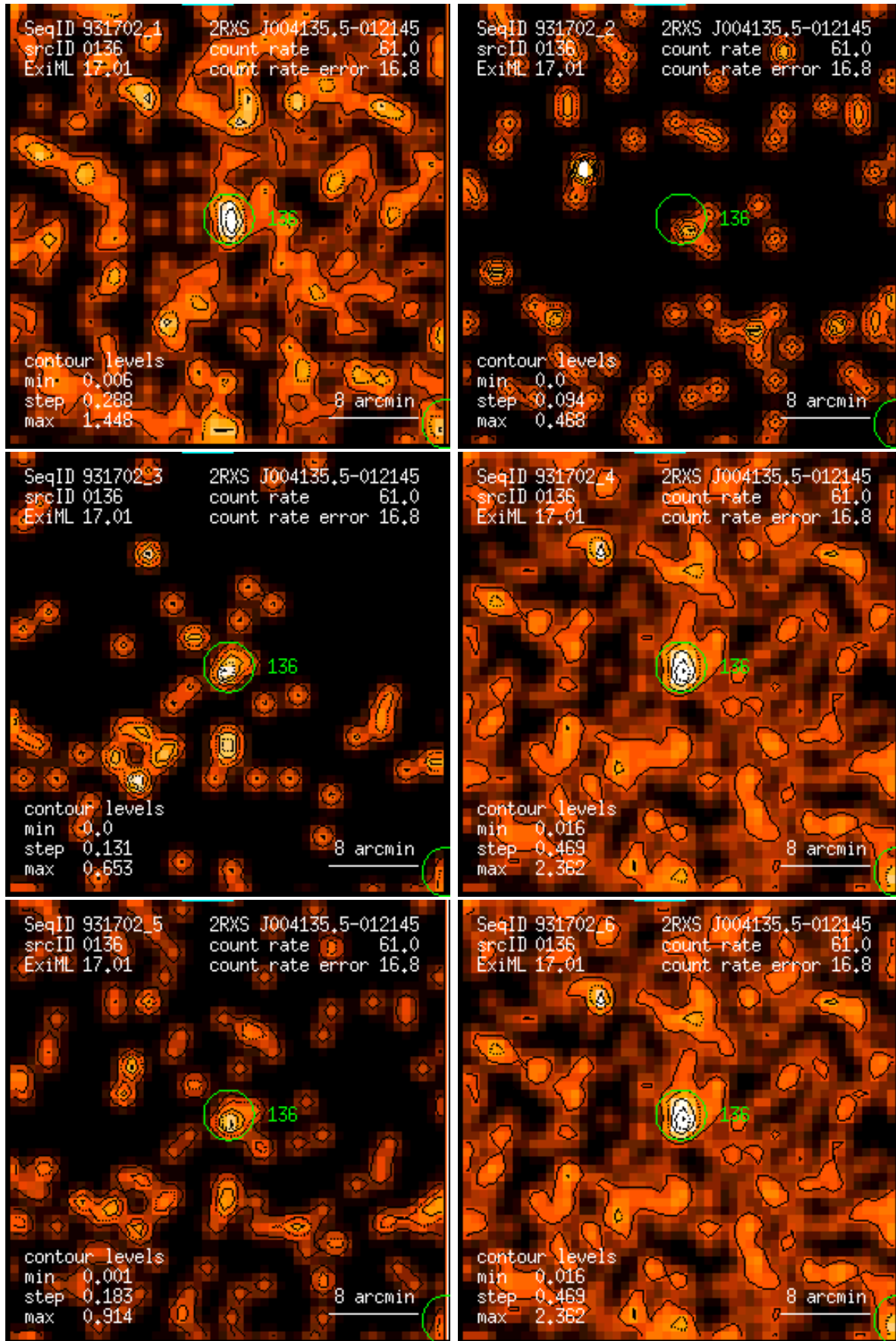
Figure 136: RASS 931702: detection 0136: band rate images, Gaussian filter: (1) PSPC channels 11 – 41, (2) 52 – 90, (3) 91 – 201, (4) 11 – 235, (5) 52 – 201, (6) 11 – 201. Broad band rates in counts/ks. Band rate contour levels in counts/ks/arcmin 2 .
