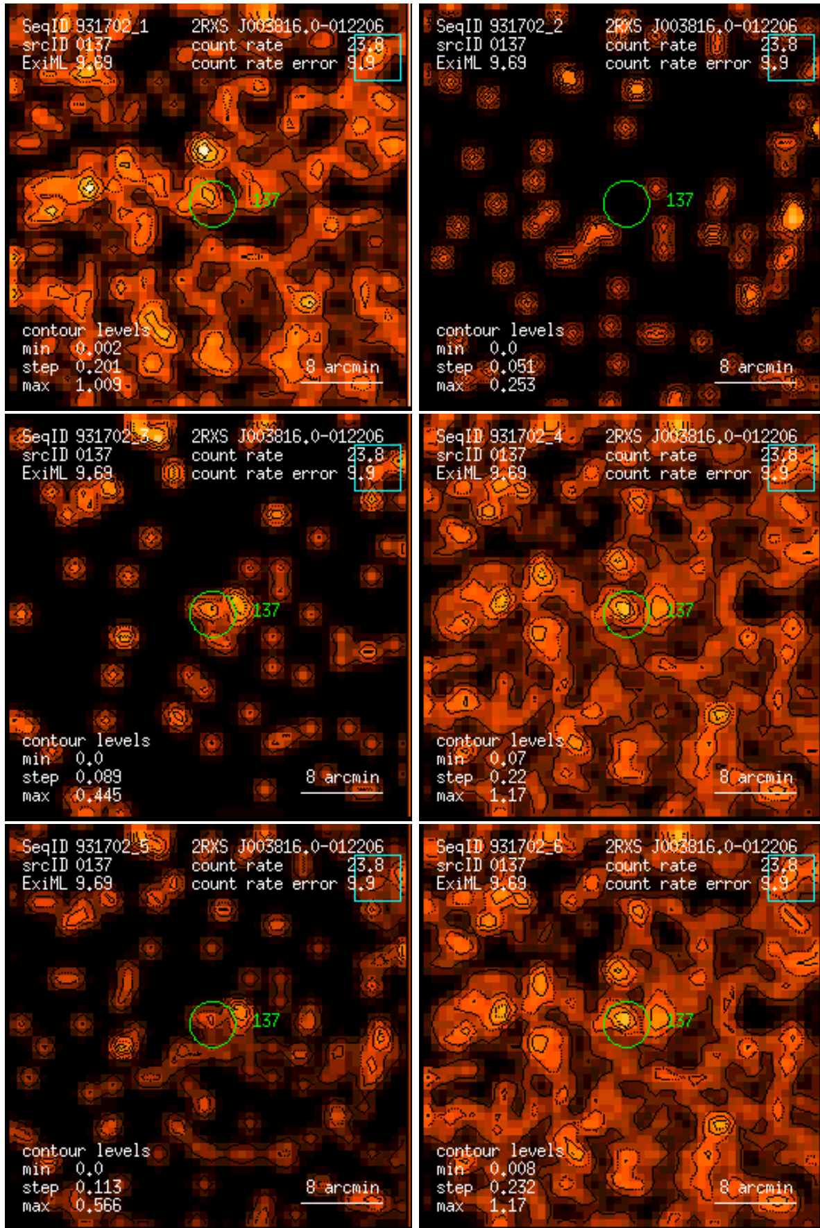
Figure 137: RASS 931702: detection 0137: band rate images, Gaussian filter: (1) PSPC channels 11 – 41, (2) 52 – 90, (3) 91 – 201, (4) 11 – 235, (5) 52 – 201, (6) 11 – 201. Broad band rates in counts/ks. Band rate contour levels in counts/ks/arcmin 2 .
