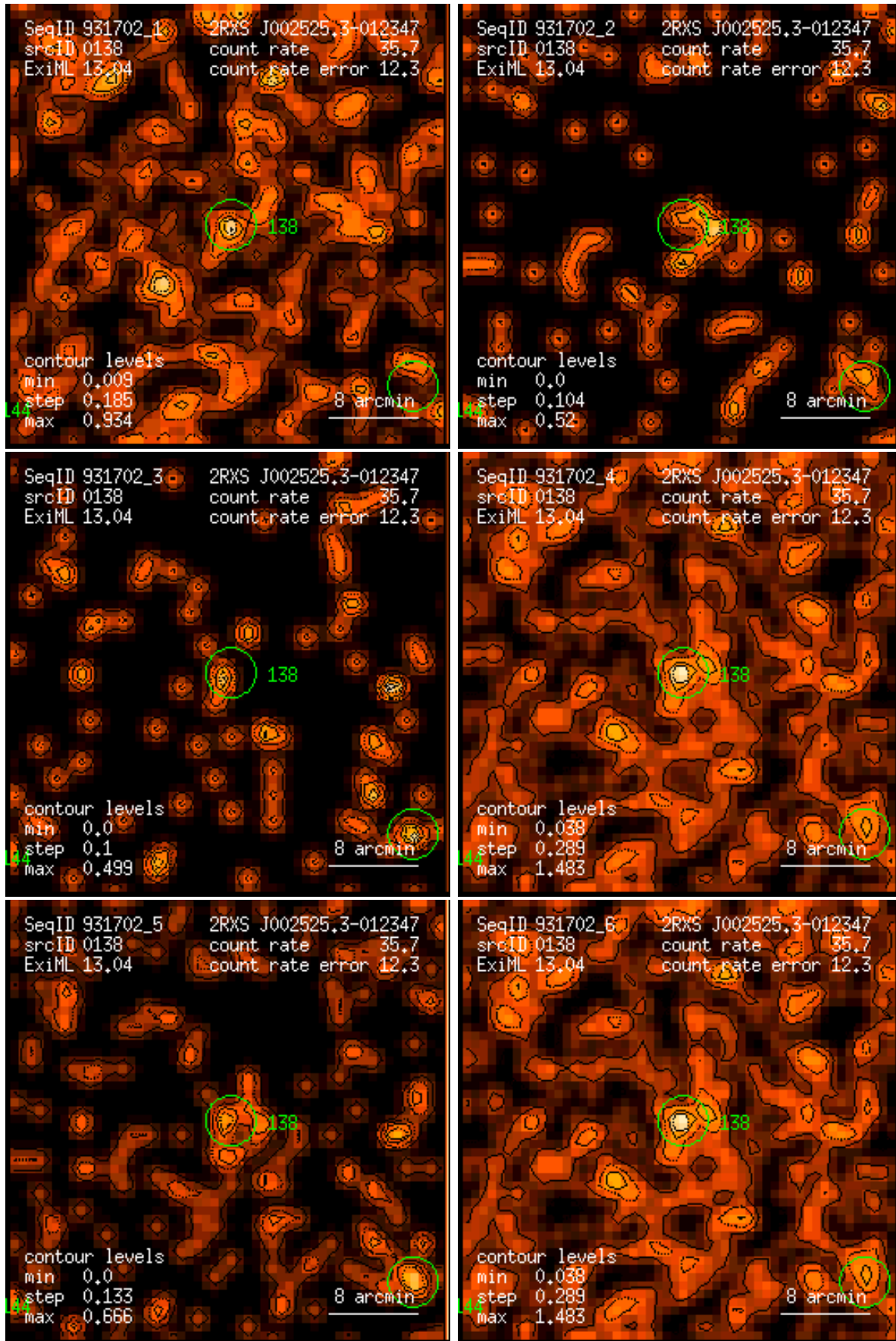
Figure 138: RASS 931702: detection 0138: band rate images, Gaussian filter: (1) PSPC channels 11 – 41, (2) 52 – 90, (3) 91 – 201, (4) 11 – 235, (5) 52 – 201, (6) 11 – 201. Broad band rates in counts/ks. Band rate contour levels in counts/ks/arcmin 2 .
