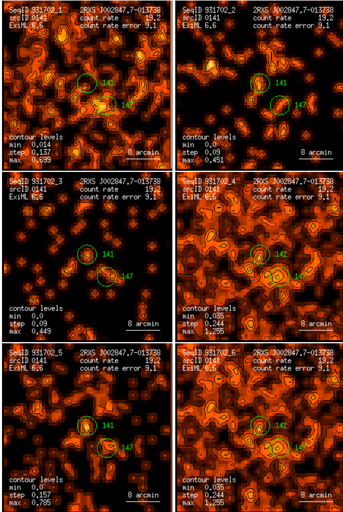
Figure 141: RASS 931702: detection 0141: band rate images, Gaussian filter: (1) PSPC channels 11 – 41, (2) 52 – 90, (3) 91 – 201, (4) 11 – 235, (5) 52 – 201, (6) 11 – 201. Broad band rates in counts/ks. Band rate contour levels in counts/ks/arcmin 2 .
