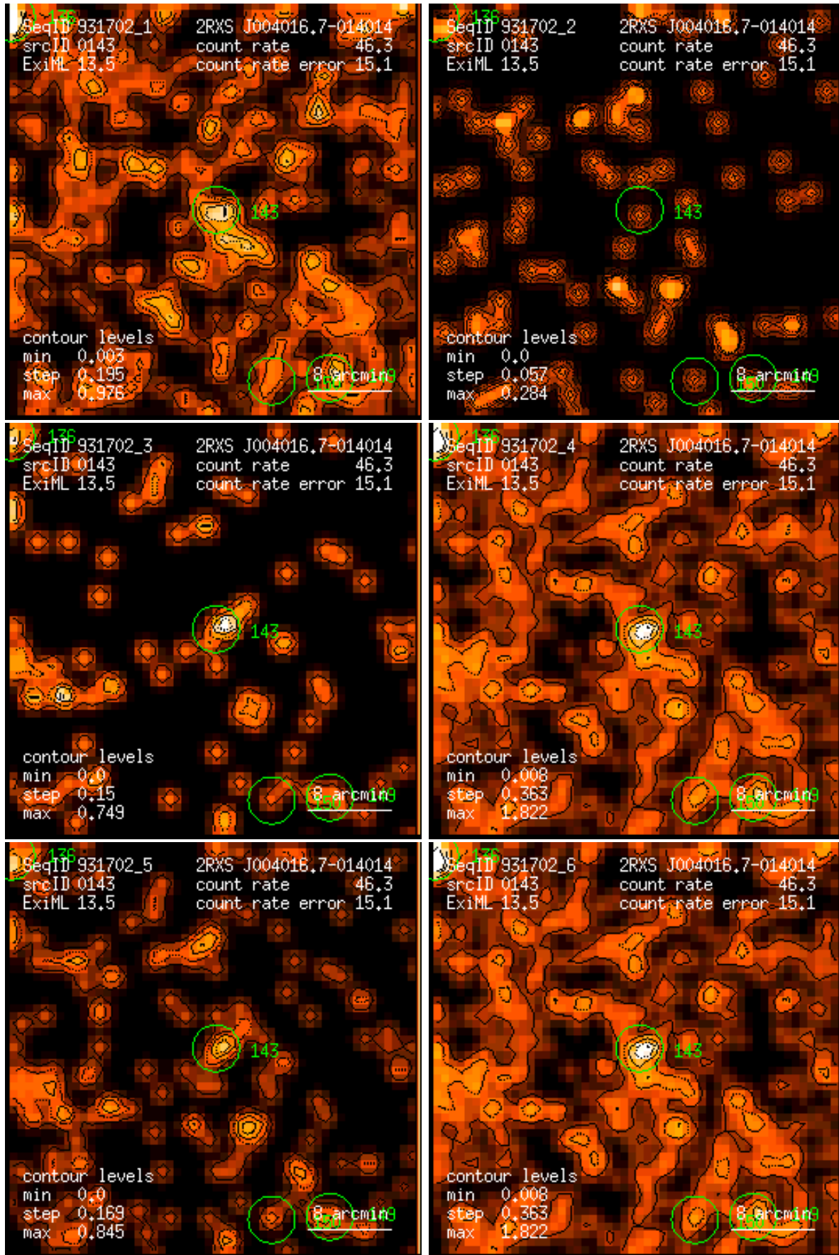
Figure 143: RASS 931702: detection 0143: band rate images, Gaussian filter: (1) PSPC channels 11 – 41, (2) 52 – 90, (3) 91 – 201, (4) 11 – 235, (5) 52 – 201, (6) 11 – 201. Broad band rates in counts/ks. Band rate contour levels in counts/ks/arcmin 2 .
