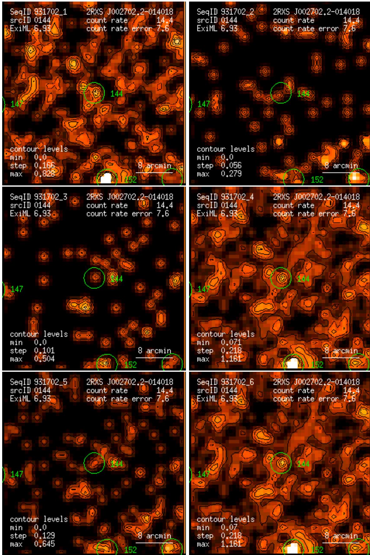
Figure 144: RASS 931702: detection 0144: band rate images, Gaussian filter: (1) PSPC channels 11 – 41, (2) 52 – 90, (3) 91 – 201, (4) 11 – 235, (5) 52 – 201, (6) 11 – 201. Broad band rates in counts/ks. Band rate contour levels in counts/ks/arcmin 2 .
