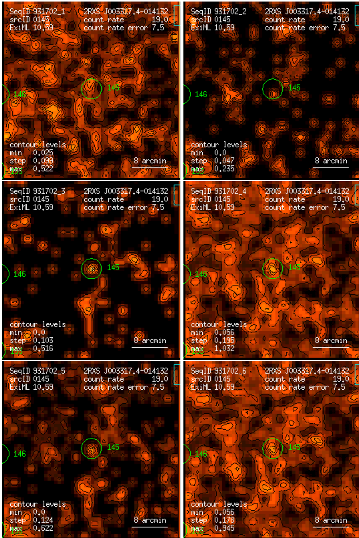
Figure 145: RASS 931702: detection 0145: band rate images, Gaussian filter: (1) PSPC channels 11 – 41, (2) 52 – 90, (3) 91 – 201, (4) 11 – 235, (5) 52 – 201, (6) 11 – 201. Broad band rates in counts/ks. Band rate contour levels in counts/ks/arcmin 2 .
