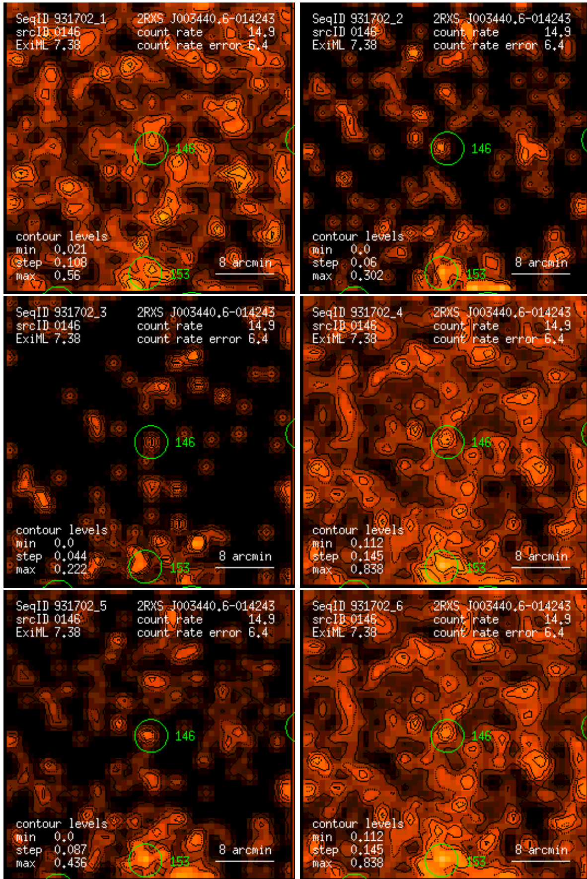
Figure 146: RASS 931702: detection 0146: band rate images, Gaussian filter: (1) PSPC channels 11 – 41, (2) 52 – 90, (3) 91 – 201, (4) 11 – 235, (5) 52 – 201, (6) 11 – 201. Broad band rates in counts/ks. Band rate contour levels in counts/ks/arcmin 2 .
