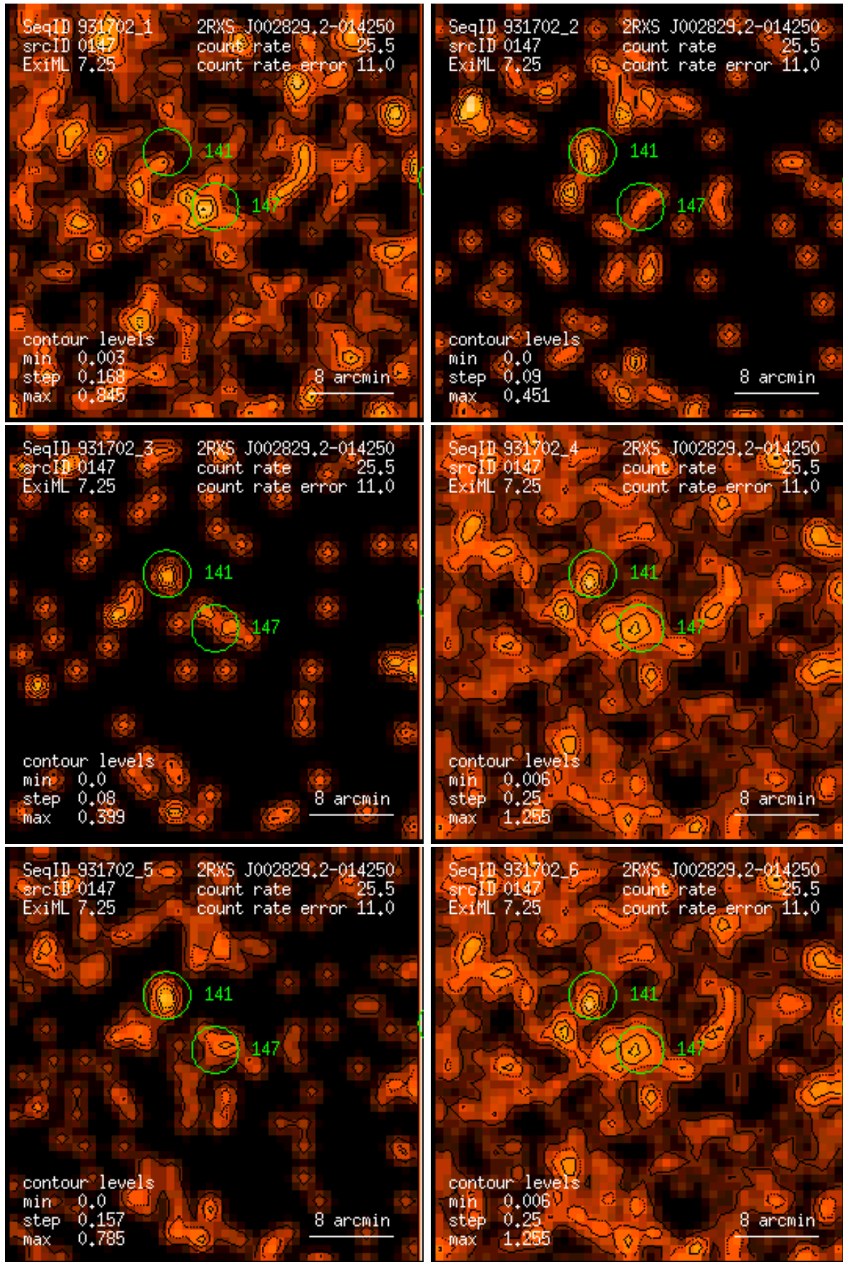
Figure 147: RASS 931702: detection 0147: band rate images, Gaussian filter: (1) PSPC channels 11 – 41, (2) 52 – 90, (3) 91 – 201, (4) 11 – 235, (5) 52 – 201, (6) 11 – 201. Broad band rates in counts/ks. Band rate contour levels in counts/ks/arcmin 2 .
