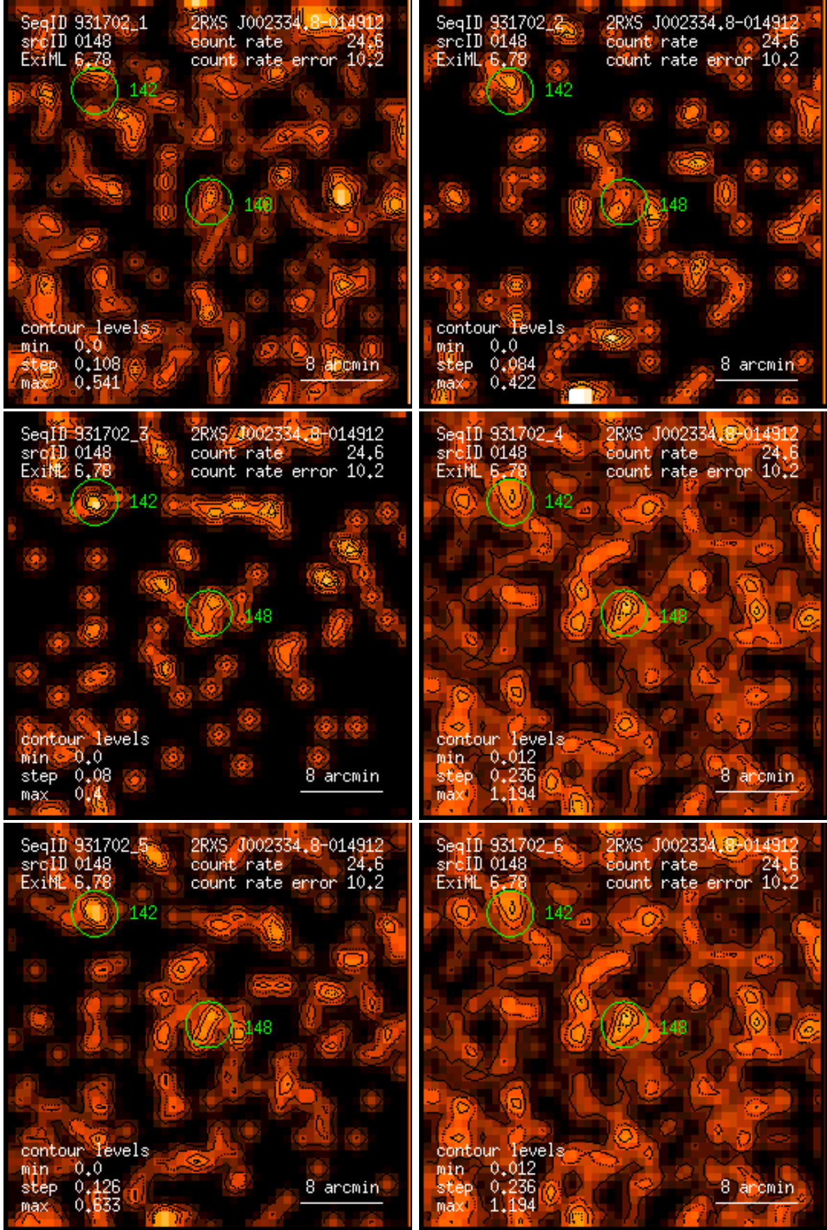
Figure 148: RASS 931702: detection 0148: band rate images, Gaussian filter: (1) PSPC channels 11 – 41, (2) 52 – 90, (3) 91 – 201, (4) 11 – 235, (5) 52 – 201, (6) 11 – 201. Broad band rates in counts/ks. Band rate contour levels in counts/ks/arcmin 2 .
