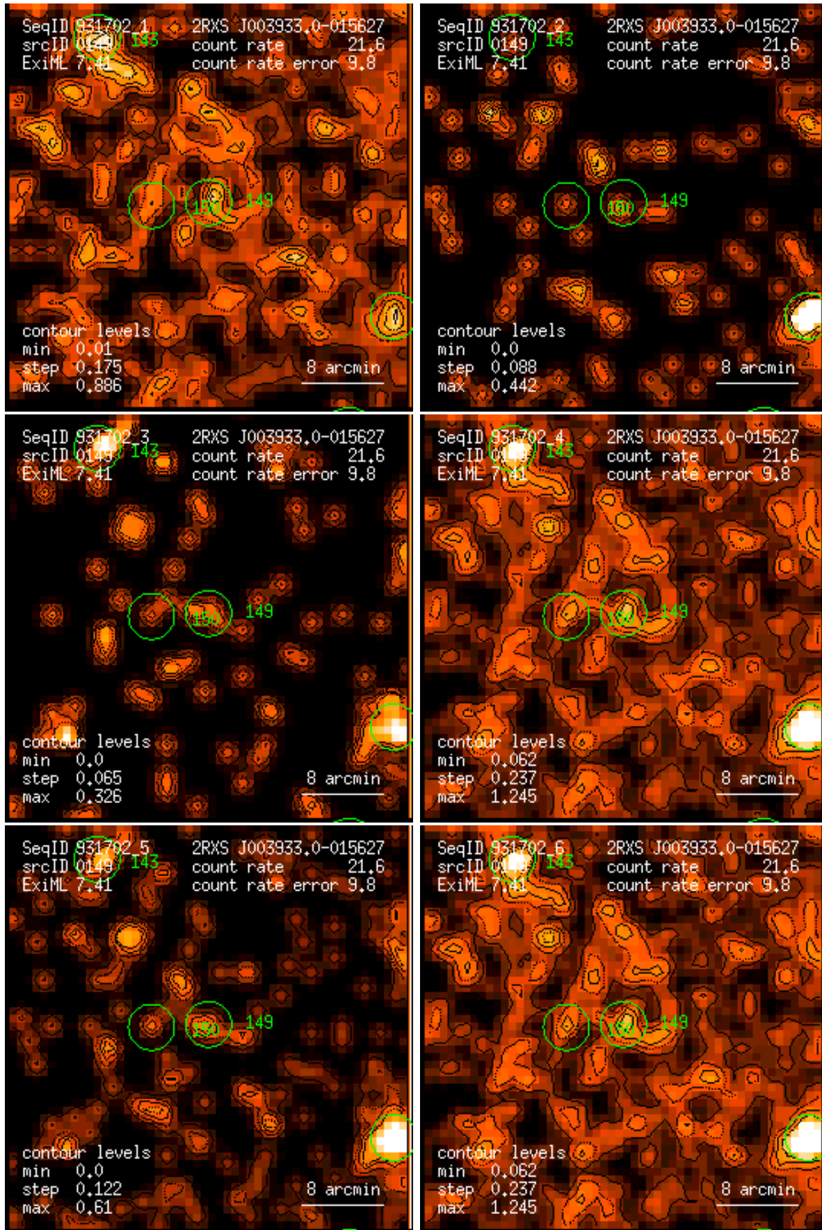
Figure 149: RASS 931702: detection 0149: band rate images, Gaussian filter: (1) PSPC channels 11 – 41, (2) 52 – 90, (3) 91 – 201, (4) 11 – 235, (5) 52 – 201, (6) 11 – 201. Broad band rates in counts/ks. Band rate contour levels in counts/ks/arcmin 2 .
