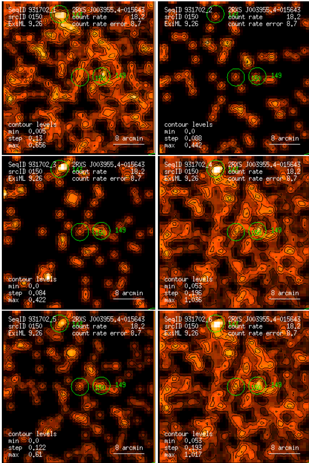
Figure 150: RASS 931702: detection 0150: band rate images, Gaussian filter: (1) PSPC channels 11 – 41, (2) 52 – 90, (3) 91 – 201, (4) 11 – 235, (5) 52 – 201, (6) 11 – 201. Broad band rates in counts/ks. Band rate contour levels in counts/ks/arcmin 2 .
