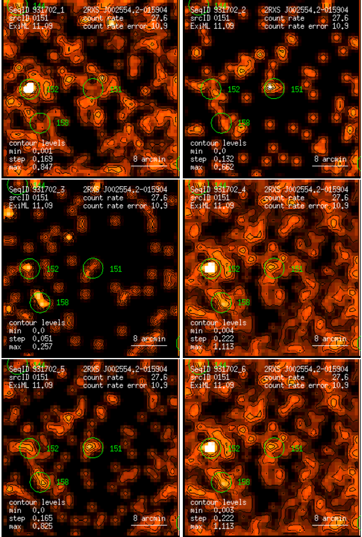
Figure 151: RASS 931702: detection 0151: band rate images, Gaussian filter: (1) PSPC channels 11 – 41, (2) 52 – 90, (3) 91 – 201, (4) 11 – 235, (5) 52 – 201, (6) 11 – 201. Broad band rates in counts/ks. Band rate contour levels in counts/ks/arcmin 2 .
