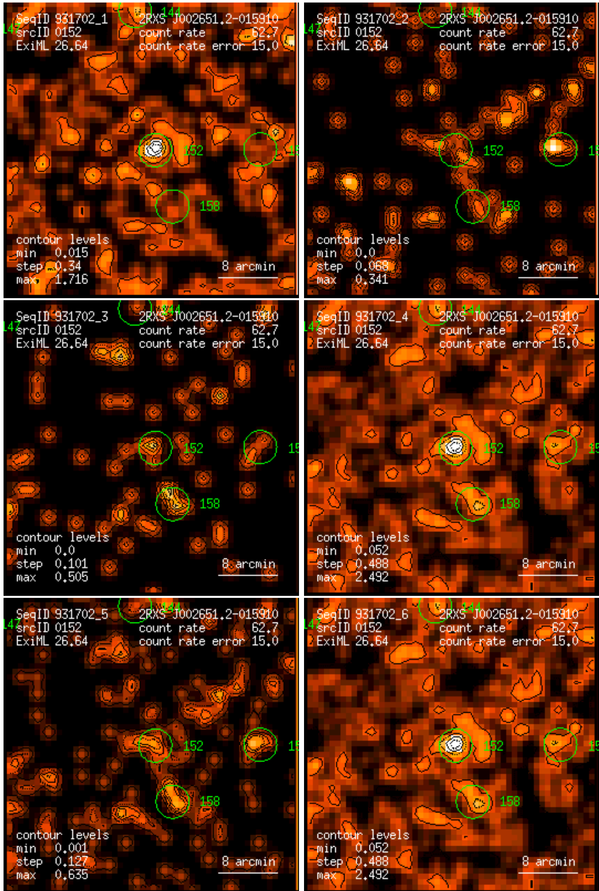
Figure 152: RASS 931702: detection 0152: band rate images, Gaussian filter: (1) PSPC channels 11 – 41, (2) 52 – 90, (3) 91 – 201, (4) 11 – 235, (5) 52 – 201, (6) 11 – 201. Broad band rates in counts/ks. Band rate contour levels in counts/ks/arcmin 2 .
