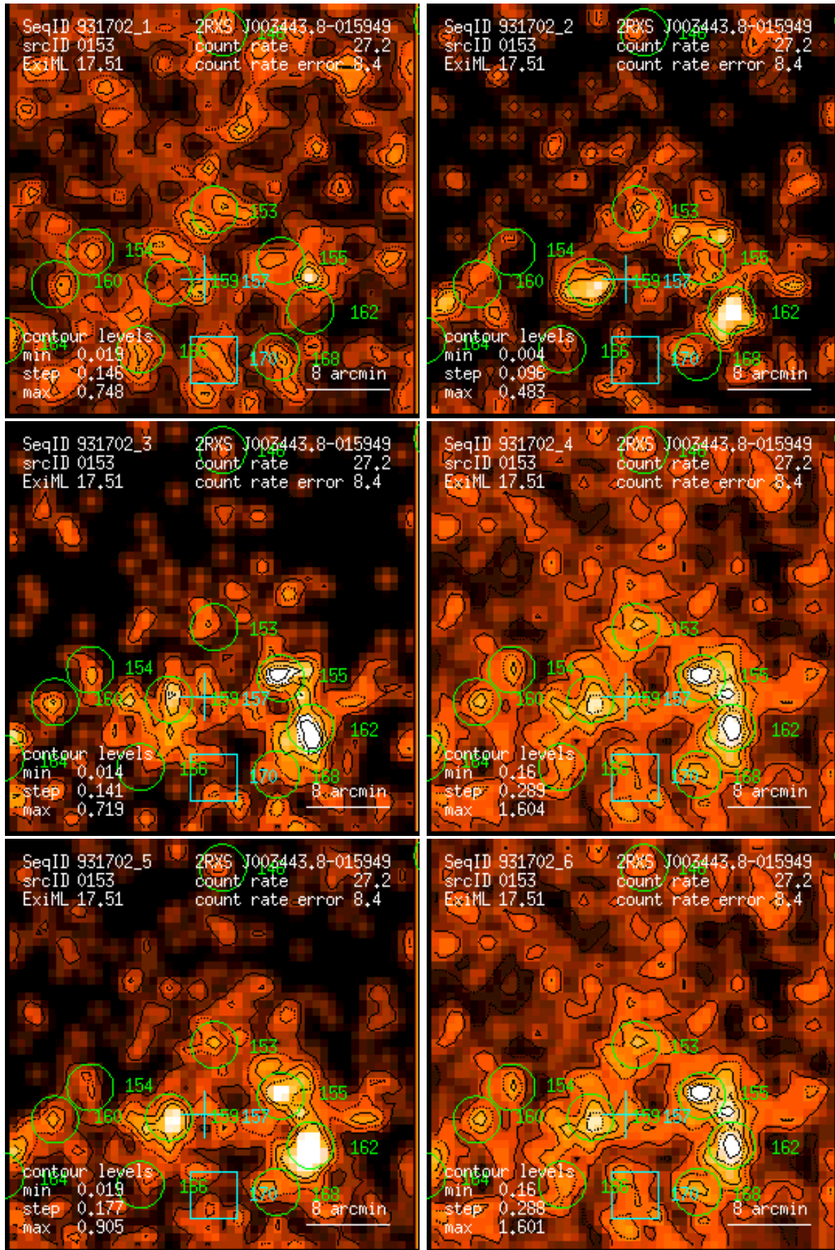
Figure 153: RASS 931702: detection 0153: band rate images, Gaussian filter: (1) PSPC channels 11 – 41, (2) 52 – 90, (3) 91 – 201, (4) 11 – 235, (5) 52 – 201, (6) 11 – 201. Broad band rates in counts/ks. Band rate contour levels in counts/ks/arcmin 2 .
