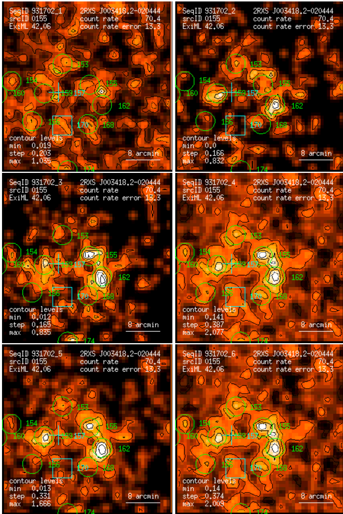
Figure 155: RASS 931702: detection 0155: band rate images, Gaussian filter: (1) PSPC channels 11 – 41, (2) 52 – 90, (3) 91 – 201, (4) 11 – 235, (5) 52 – 201, (6) 11 – 201. Broad band rates in counts/ks. Band rate contour levels in counts/ks/arcmin 2 .
