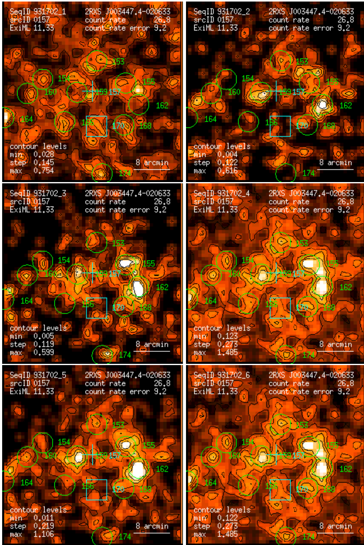
Figure 157: RASS 931702: detection 0157: band rate images, Gaussian filter: (1) PSPC channels 11 – 41, (2) 52 – 90, (3) 91 – 201, (4) 11 – 235, (5) 52 – 201, (6) 11 – 201. Broad band rates in counts/ks. Band rate contour levels in counts/ks/arcmin 2 .
