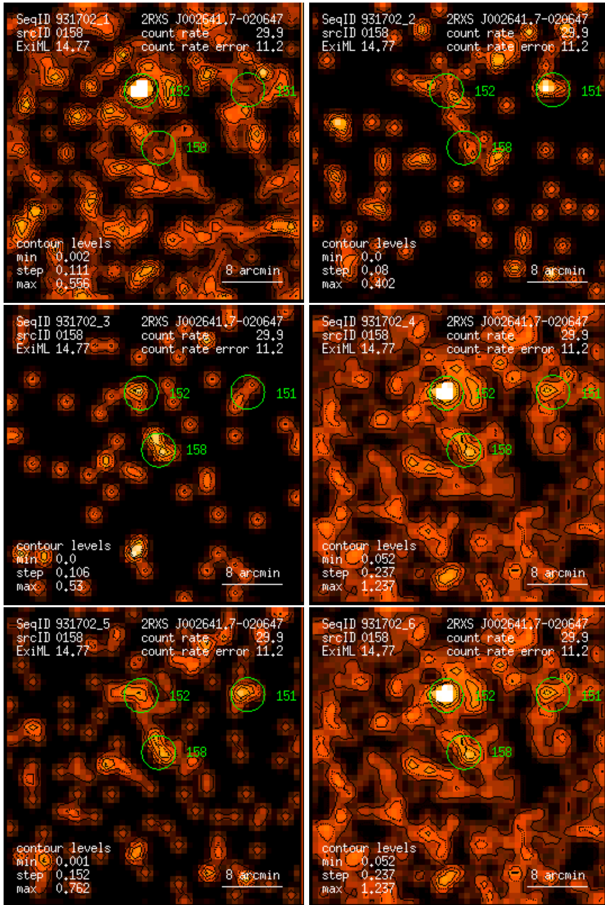
Figure 158: RASS 931702: detection 0158: band rate images, Gaussian filter: (1) PSPC channels 11 – 41, (2) 52 – 90, (3) 91 – 201, (4) 11 – 235, (5) 52 – 201, (6) 11 – 201. Broad band rates in counts/ks. Band rate contour levels in counts/ks/arcmin 2 .
