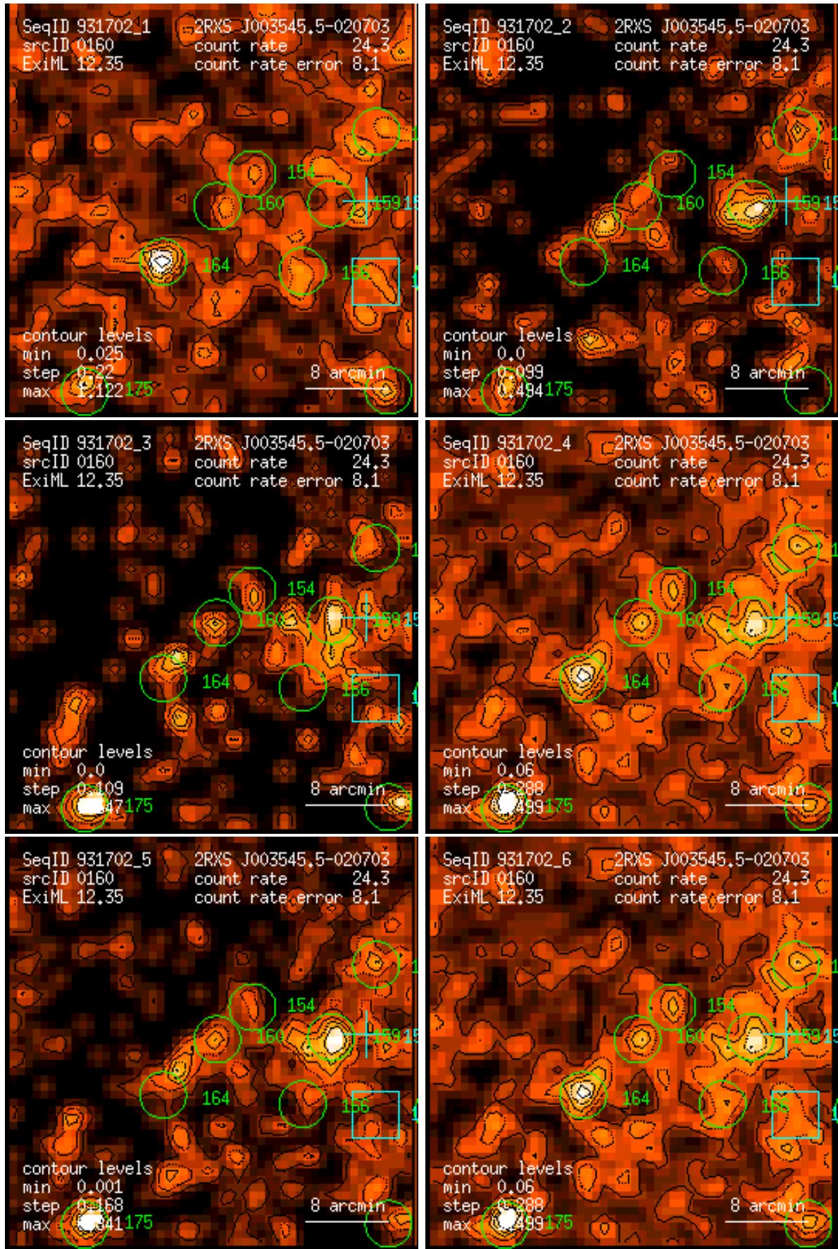
Figure 160: RASS 931702: detection 0160: band rate images, Gaussian filter: (1) PSPC channels 11 – 41, (2) 52 – 90, (3) 91 – 201, (4) 11 – 235, (5) 52 – 201, (6) 11 – 201. Broad band rates in counts/ks. Band rate contour levels in counts/ks/arcmin 2 .
