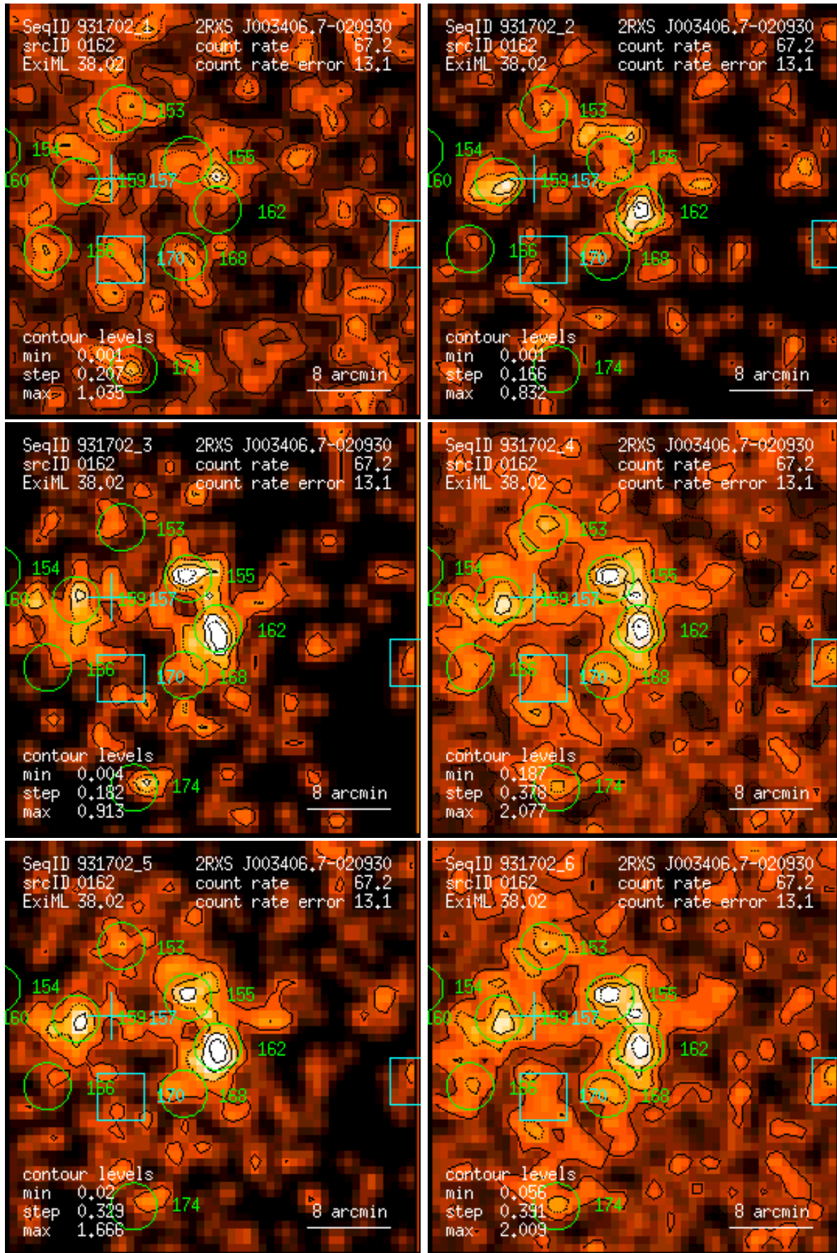
Figure 162: RASS 931702: detection 0162: band rate images, Gaussian filter: (1) PSPC channels 11 – 41, (2) 52 – 90, (3) 91 – 201, (4) 11 – 235, (5) 52 – 201, (6) 11 – 201. Broad band rates in counts/ks. Band rate contour levels in counts/ks/arcmin 2 .
