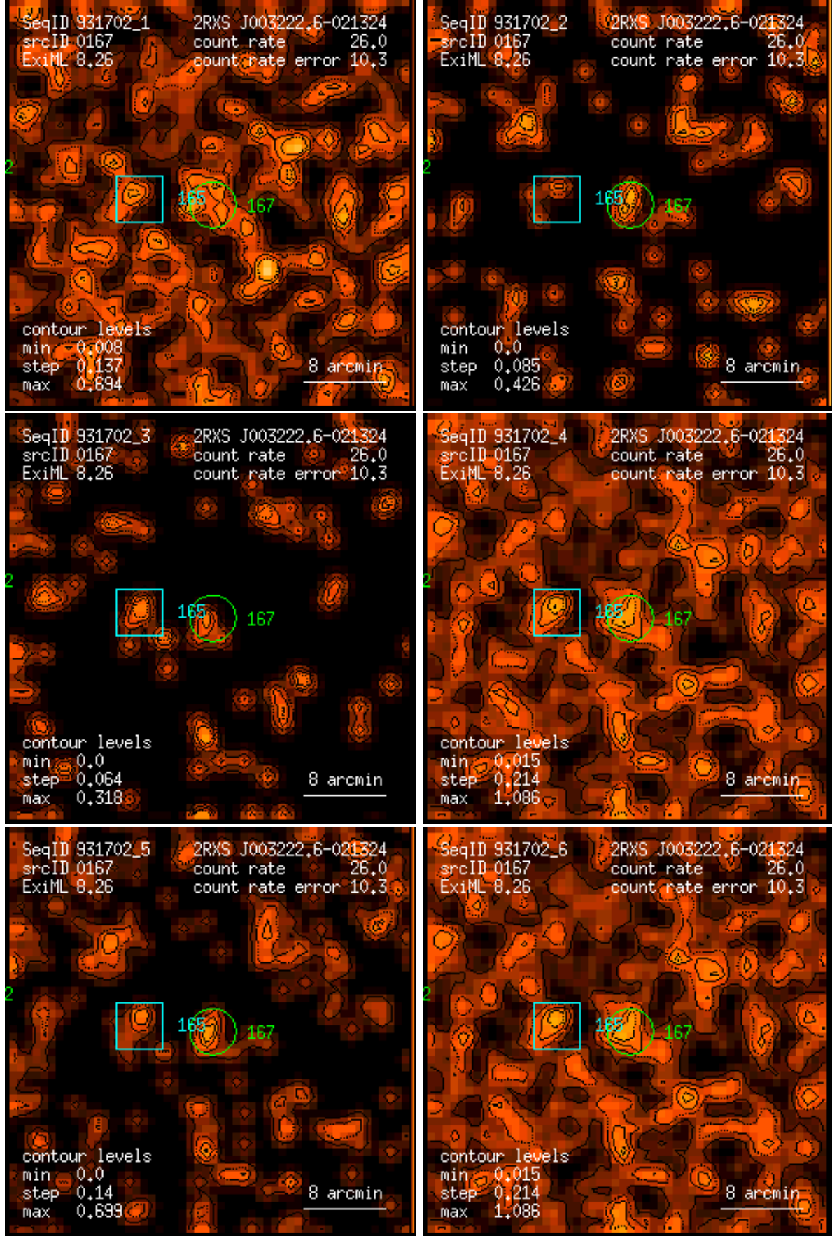
Figure 167: RASS 931702: detection 0167: band rate images, Gaussian filter: (1) PSPC channels 11 – 41, (2) 52 – 90, (3) 91 – 201, (4) 11 – 235, (5) 52 – 201, (6) 11 – 201. Broad band rates in counts/ks. Band rate contour levels in counts/ks/arcmin 2 .
