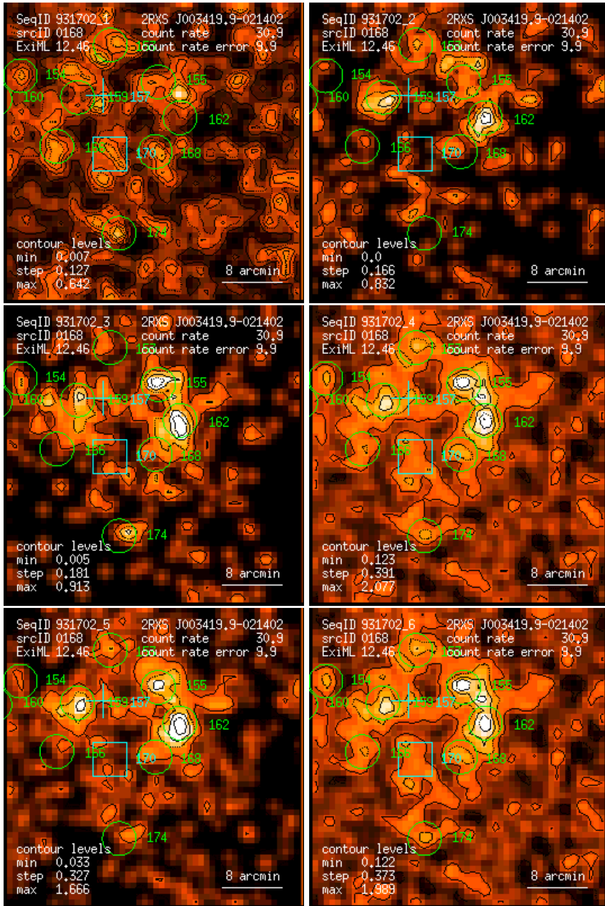
Figure 168: RASS 931702: detection 0168: band rate images, Gaussian filter: (1) PSPC channels 11 – 41, (2) 52 – 90, (3) 91 – 201, (4) 11 – 235, (5) 52 – 201, (6) 11 – 201. Broad band rates in counts/ks. Band rate contour levels in counts/ks/arcmin 2 .
