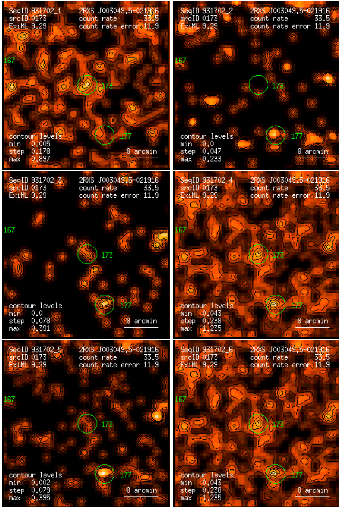
Figure 173: RASS 931702: detection 0173: band rate images, Gaussian filter: (1) PSPC channels 11 – 41, (2) 52 – 90, (3) 91 – 201, (4) 11 – 235, (5) 52 – 201, (6) 11 – 201. Broad band rates in counts/ks. Band rate contour levels in counts/ks/arcmin 2 .
