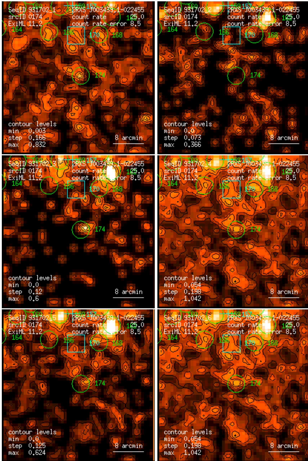
Figure 174: RASS 931702: detection 0174: band rate images, Gaussian filter: (1) PSPC channels 11 – 41, (2) 52 – 90, (3) 91 – 201, (4) 11 – 235, (5) 52 – 201, (6) 11 – 201. Broad band rates in counts/ks. Band rate contour levels in counts/ks/arcmin 2 .
