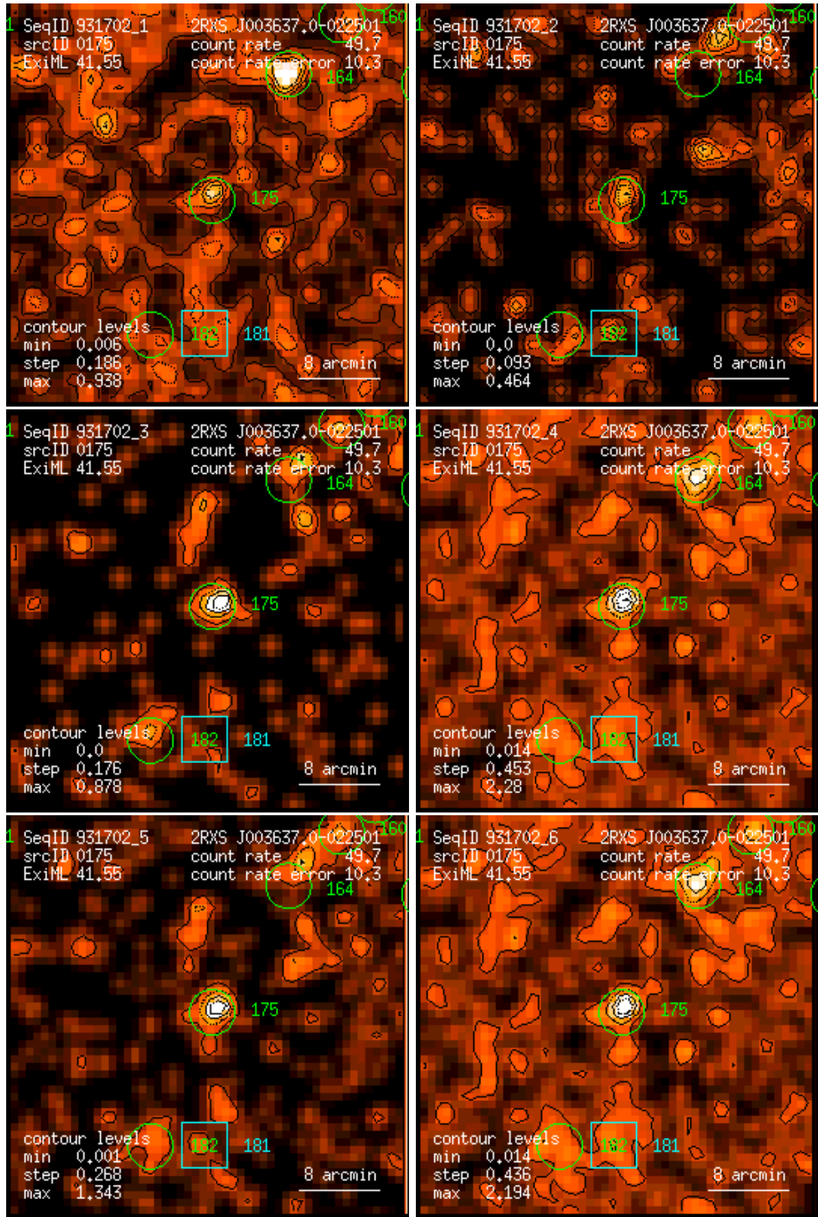
Figure 175: RASS 931702: detection 0175: band rate images, Gaussian filter: (1) PSPC channels 11 – 41, (2) 52 – 90, (3) 91 – 201, (4) 11 – 235, (5) 52 – 201, (6) 11 – 201. Broad band rates in counts/ks. Band rate contour levels in counts/ks/arcmin 2 .
