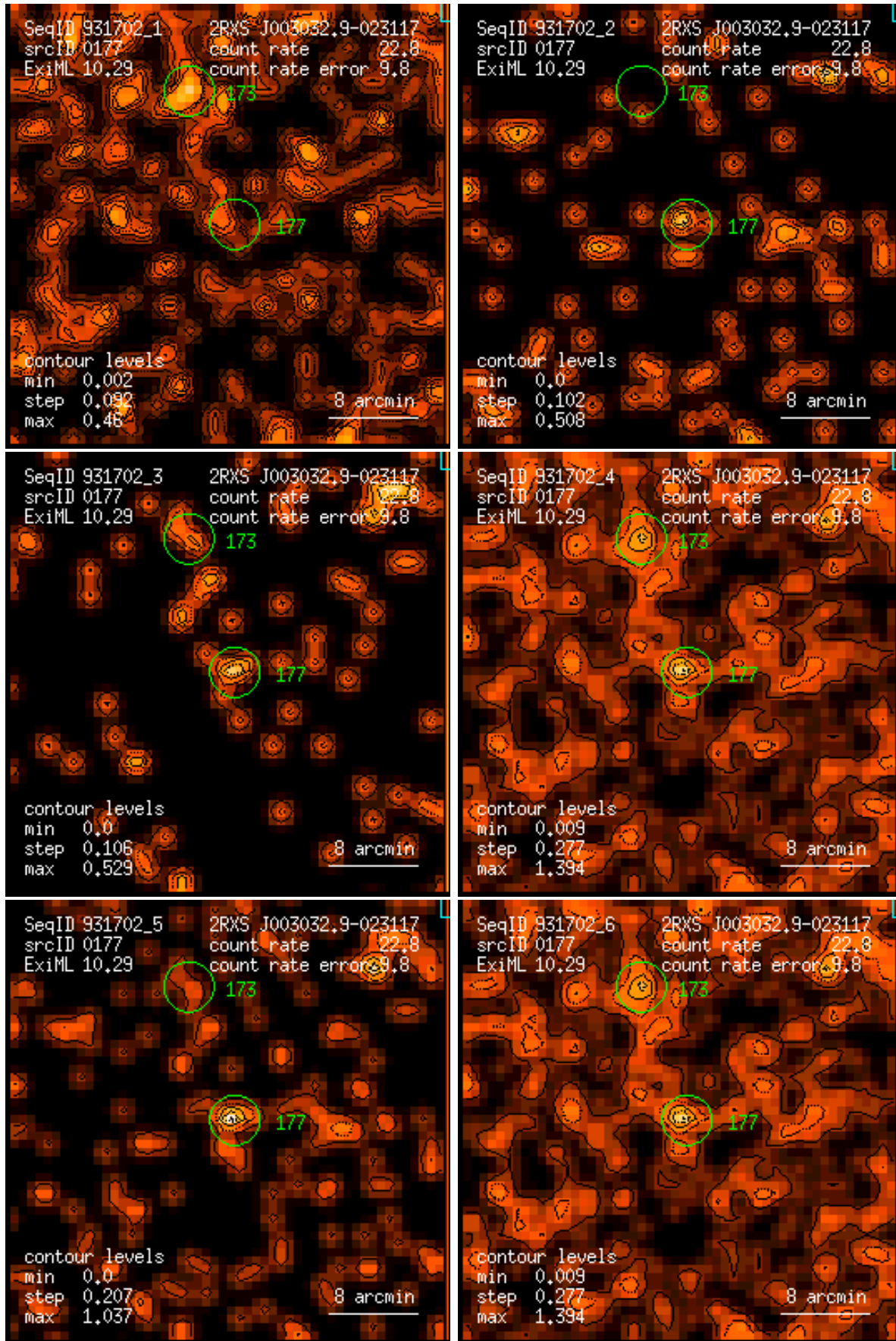
Figure 177: RASS 931702: detection 0177: band rate images, Gaussian filter: (1) PSPC channels 11 – 41, (2) 52 – 90, (3) 91 – 201, (4) 11 – 235, (5) 52 – 201, (6) 11 – 201. Broad band rates in counts/ks. Band rate contour levels in counts/ks/arcmin 2 .
