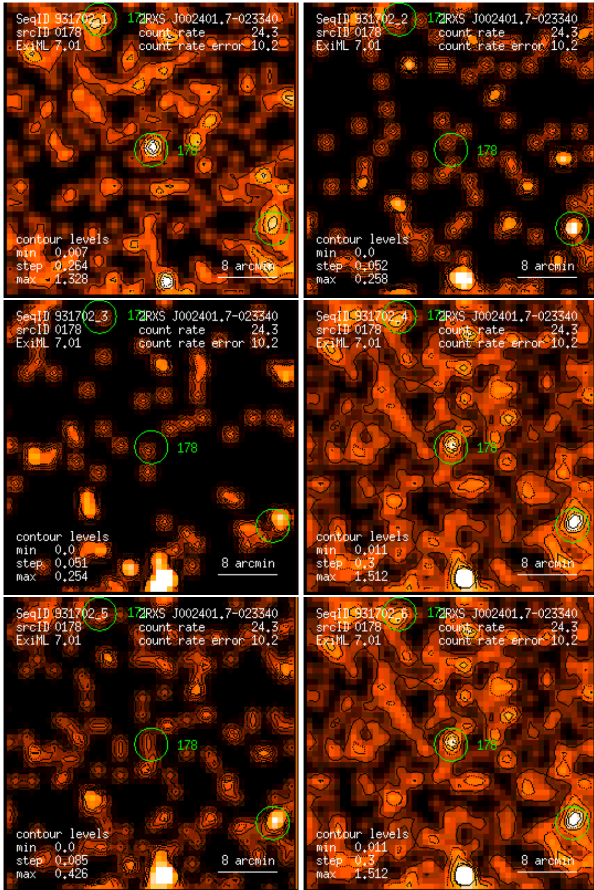
Figure 178: RASS 931702: detection 0178: band rate images, Gaussian filter: (1) PSPC channels 11 – 41, (2) 52 – 90, (3) 91 – 201, (4) 11 – 235, (5) 52 – 201, (6) 11 – 201. Broad band rates in counts/ks. Band rate contour levels in counts/ks/arcmin 2 .
