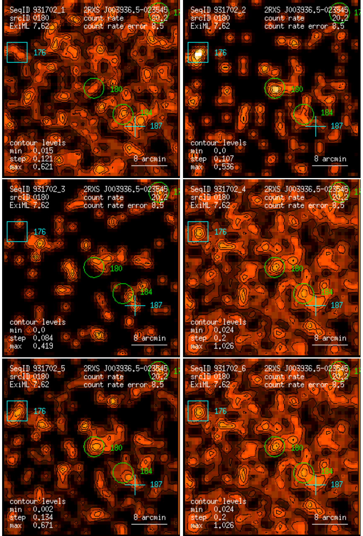
Figure 180: RASS 931702: detection 0180: band rate images, Gaussian filter: (1) PSPC channels 11 – 41, (2) 52 – 90, (3) 91 – 201, (4) 11 – 235, (5) 52 – 201, (6) 11 – 201. Broad band rates in counts/ks. Band rate contour levels in counts/ks/arcmin 2 .
