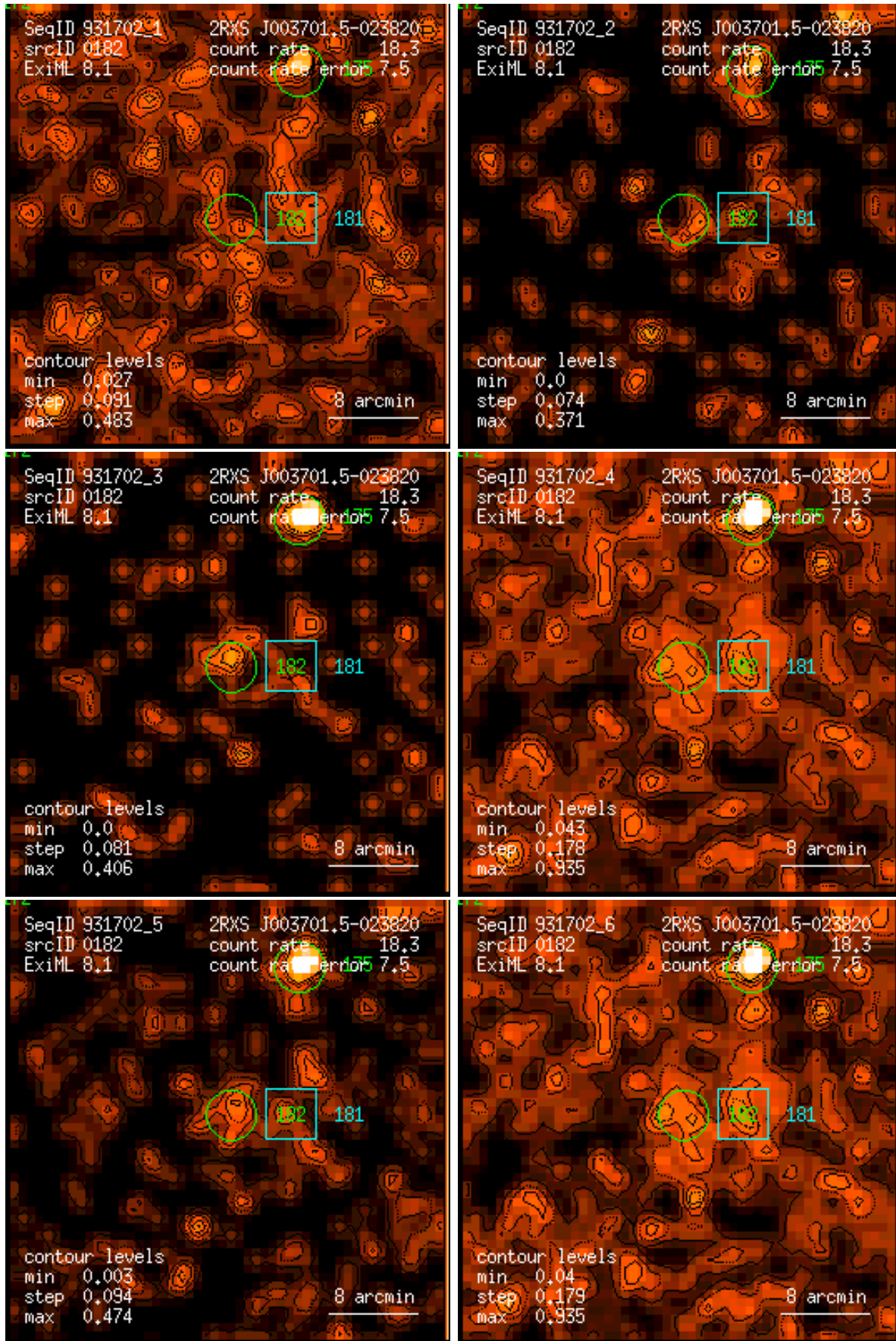
Figure 182: RASS 931702: detection 0182: band rate images, Gaussian filter: (1) PSPC channels 11 – 41, (2) 52 – 90, (3) 91 – 201, (4) 11 – 235, (5) 52 – 201, (6) 11 – 201. Broad band rates in counts/ks. Band rate contour levels in counts/ks/arcmin 2 .
