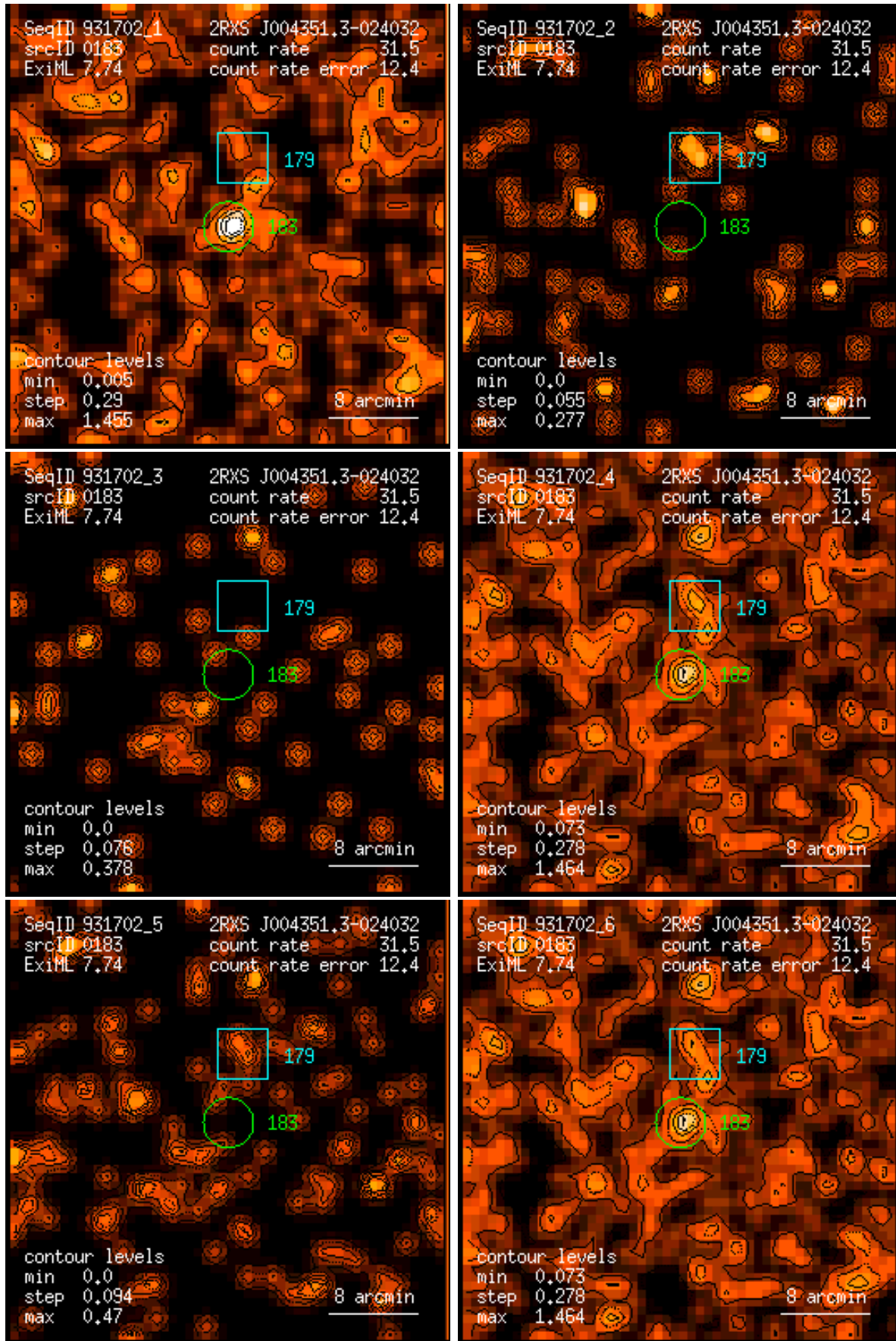
Figure 183: RASS 931702: detection 0183: band rate images, Gaussian filter: (1) PSPC channels 11 – 41, (2) 52 – 90, (3) 91 – 201, (4) 11 – 235, (5) 52 – 201, (6) 11 – 201. Broad band rates in counts/ks. Band rate contour levels in counts/ks/arcmin 2 .
