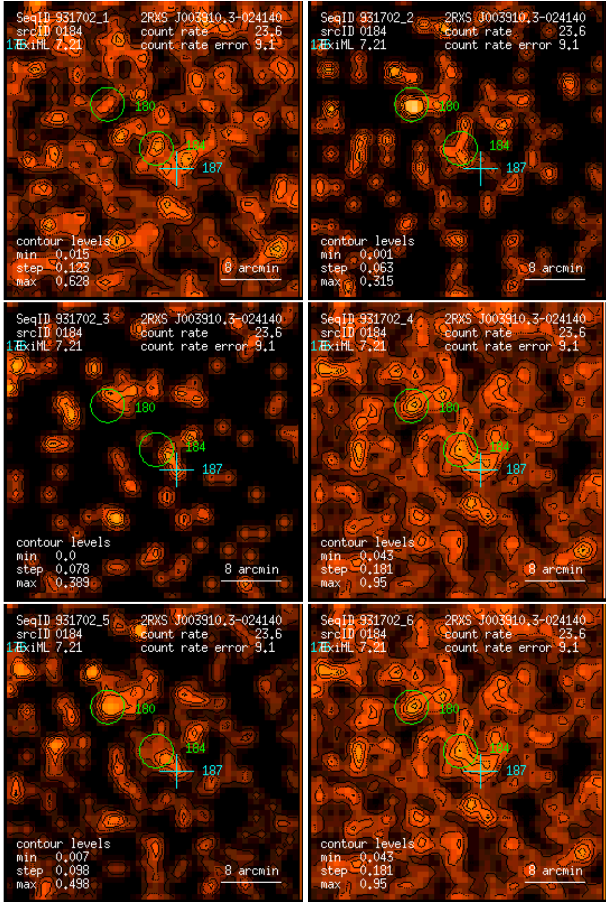
Figure 184: RASS 931702: detection 0184: band rate images, Gaussian filter: (1) PSPC channels 11 – 41, (2) 52 – 90, (3) 91 – 201, (4) 11 – 235, (5) 52 – 201, (6) 11 – 201. Broad band rates in counts/ks. Band rate contour levels in counts/ks/arcmin 2 .
