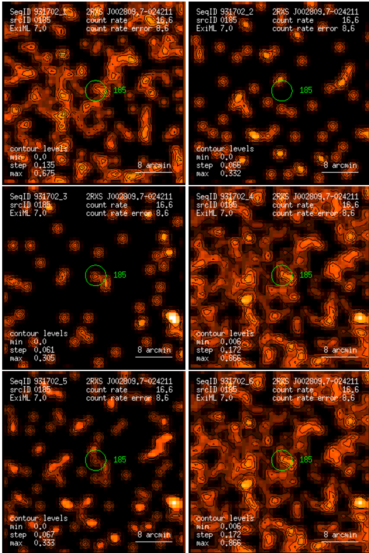
Figure 185: RASS 931702: detection 0185: band rate images, Gaussian filter: (1) PSPC channels 11 – 41, (2) 52 – 90, (3) 91 – 201, (4) 11 – 235, (5) 52 – 201, (6) 11 – 201. Broad band rates in counts/ks. Band rate contour levels in counts/ks/arcmin 2 .
