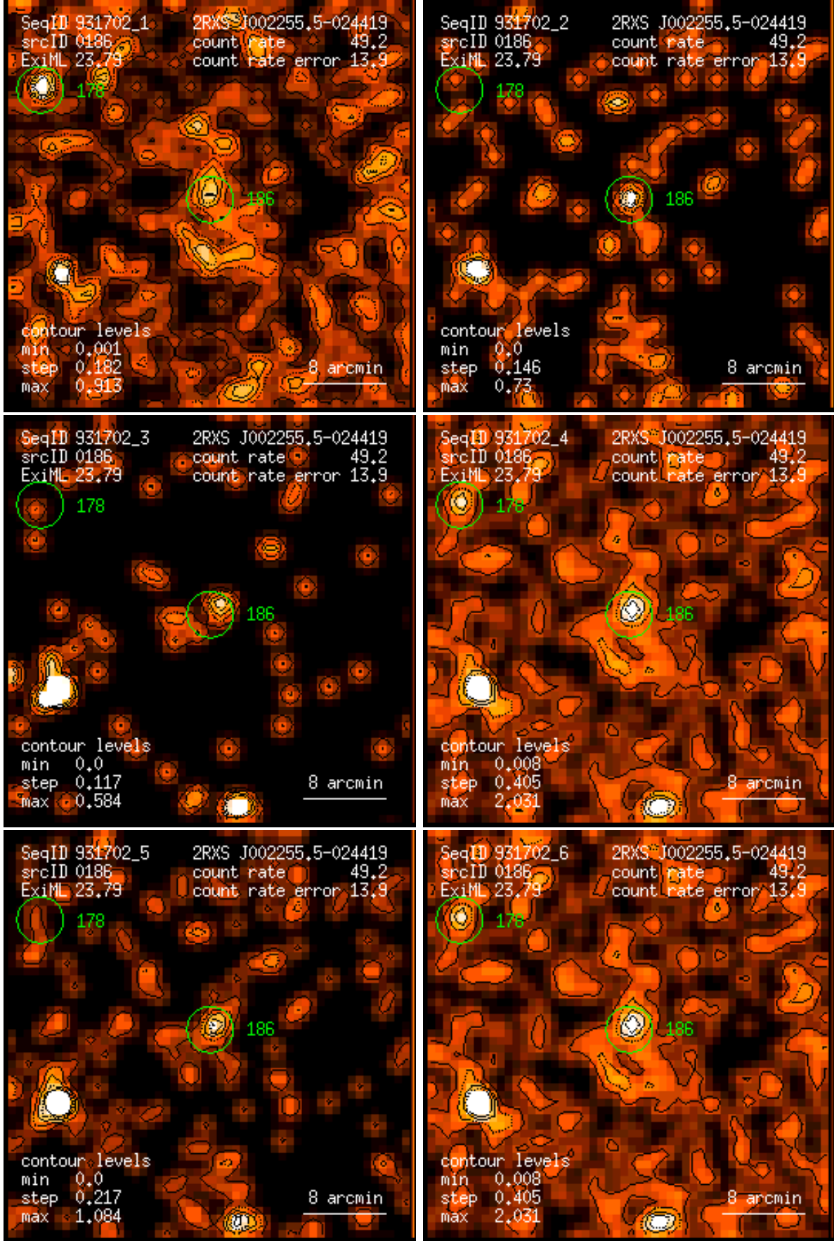
Figure 186: RASS 931702: detection 0186: band rate images, Gaussian filter: (1) PSPC channels 11 – 41, (2) 52 – 90, (3) 91 – 201, (4) 11 – 235, (5) 52 – 201, (6) 11 – 201. Broad band rates in counts/ks. Band rate contour levels in counts/ks/arcmin 2 .
