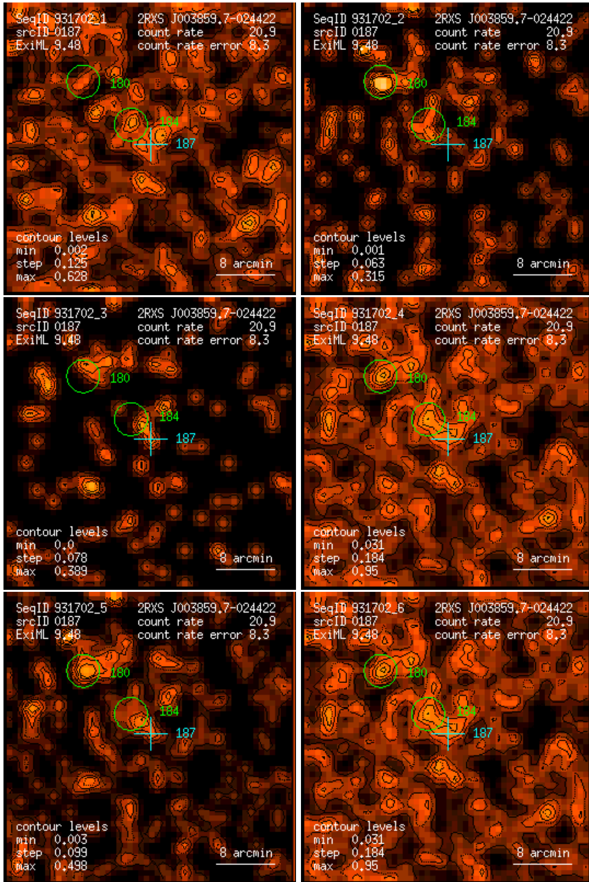
Figure 187: RASS 931702: detection 0187: band rate images, Gaussian filter: (1) PSPC channels 11 – 41, (2) 52 – 90, (3) 91 – 201, (4) 11 – 235, (5) 52 – 201, (6) 11 – 201. Broad band rates in counts/ks. Band rate contour levels in counts/ks/arcmin 2 .
