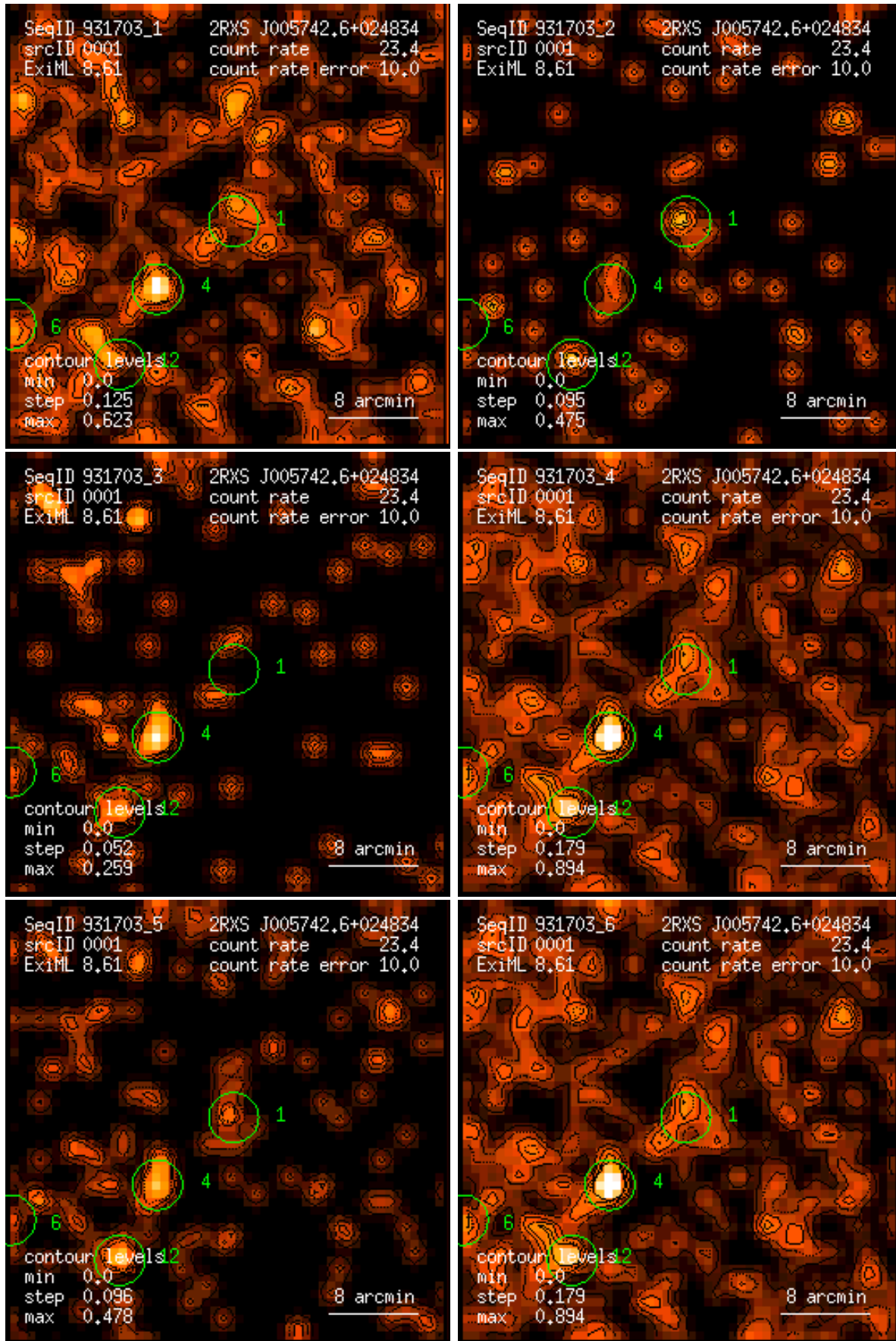
Figure 1: RASS 931703: detection 0001: band rate images, Gaussian filter: (1) PSPC channels 11 – 41, (2) 52 – 90, (3) 91 – 201, (4) 11 – 235, (5) 52 – 201, (6) 11 – 201. Broad band rates in counts/ks. Band rate contour levels in counts/ks/arcmin 2 .
