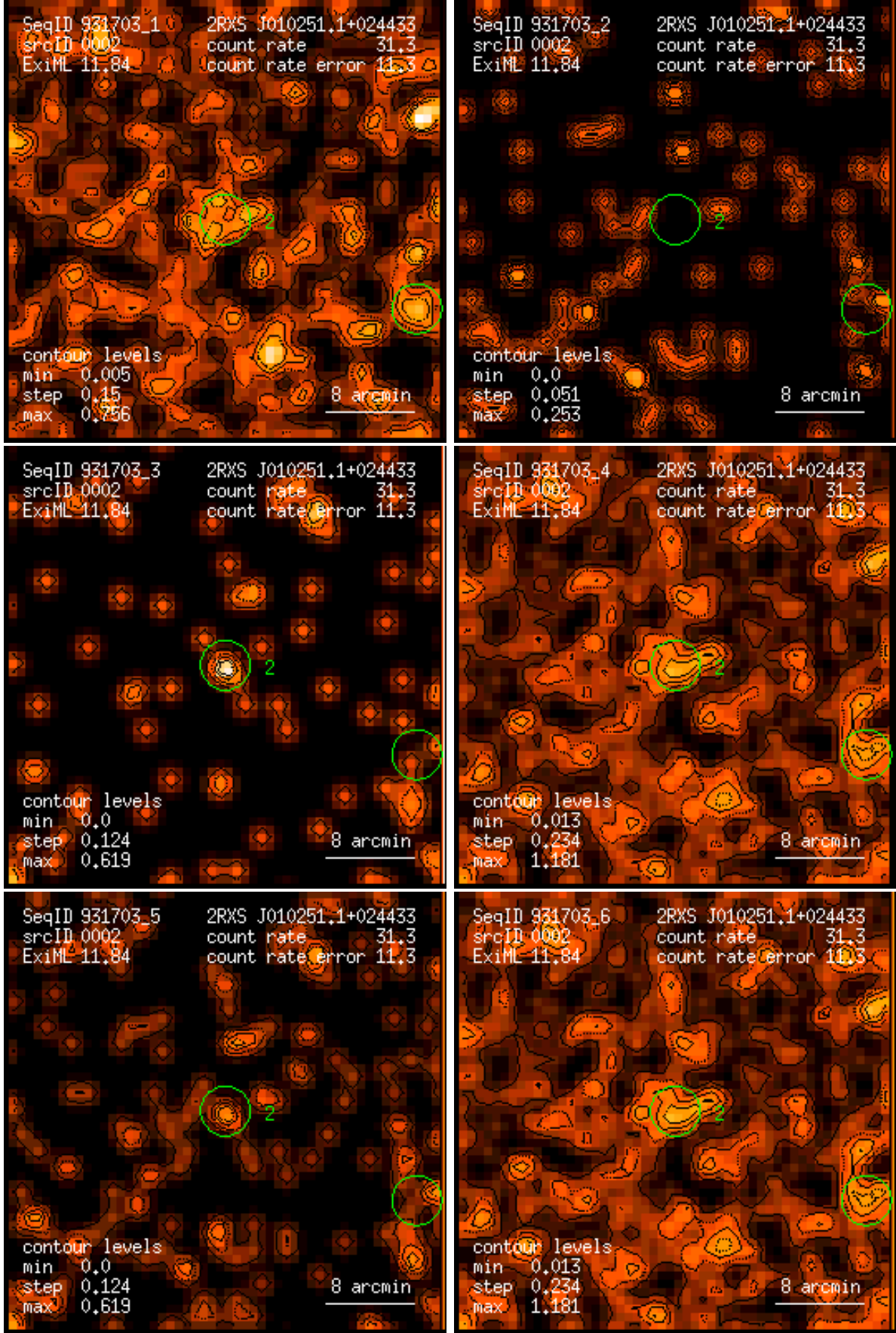
Figure 2: RASS 931703: detection 0002: band rate images, Gaussian filter: (1) PSPC channels 11 – 41, (2) 52 – 90, (3) 91 – 201, (4) 11 – 235, (5) 52 – 201, (6) 11 – 201. Broad band rates in counts/ks. Band rate contour levels in counts/ks/arcmin 2 .
