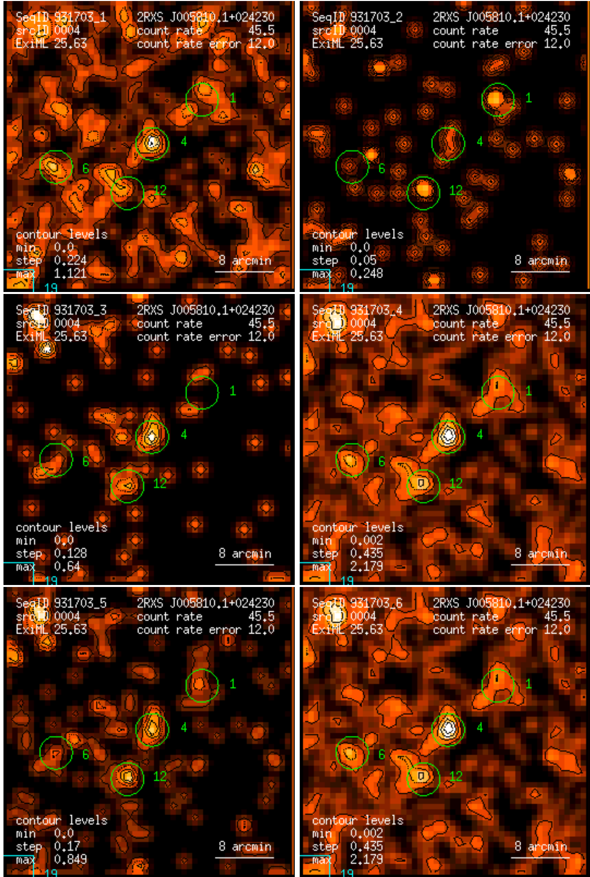
Figure 4: RASS 931703: detection 0004: band rate images, Gaussian filter: (1) PSPC channels 11 – 41, (2) 52 – 90, (3) 91 – 201, (4) 11 – 235, (5) 52 – 201, (6) 11 – 201. Broad band rates in counts/ks. Band rate contour levels in counts/ks/arcmin 2 .
