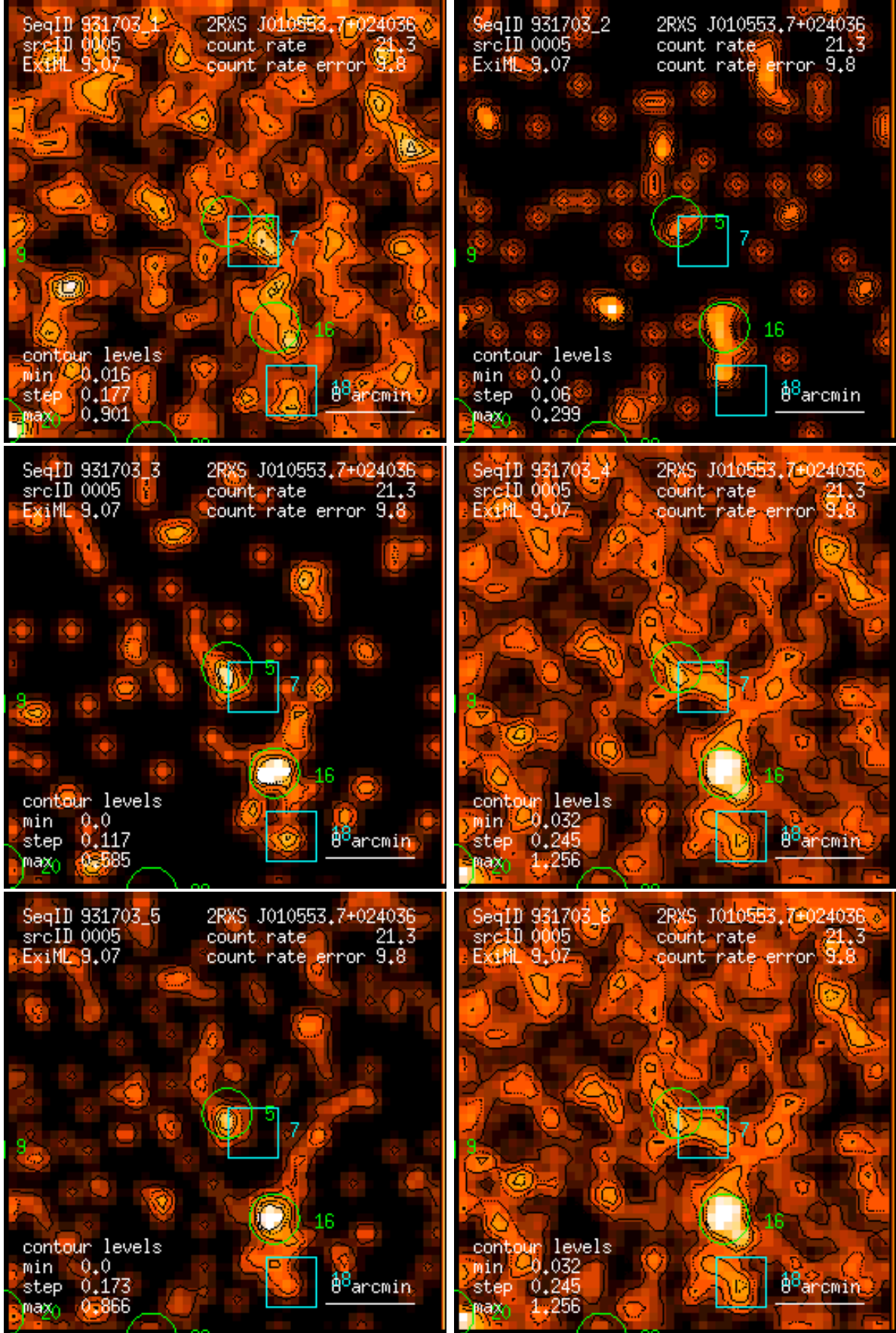
Figure 5: RASS 931703: detection 0005: band rate images, Gaussian filter: (1) PSPC channels 11 – 41, (2) 52 – 90, (3) 91 – 201, (4) 11 – 235, (5) 52 – 201, (6) 11 – 201. Broad band rates in counts/ks. Band rate contour levels in counts/ks/arcmin 2 .
