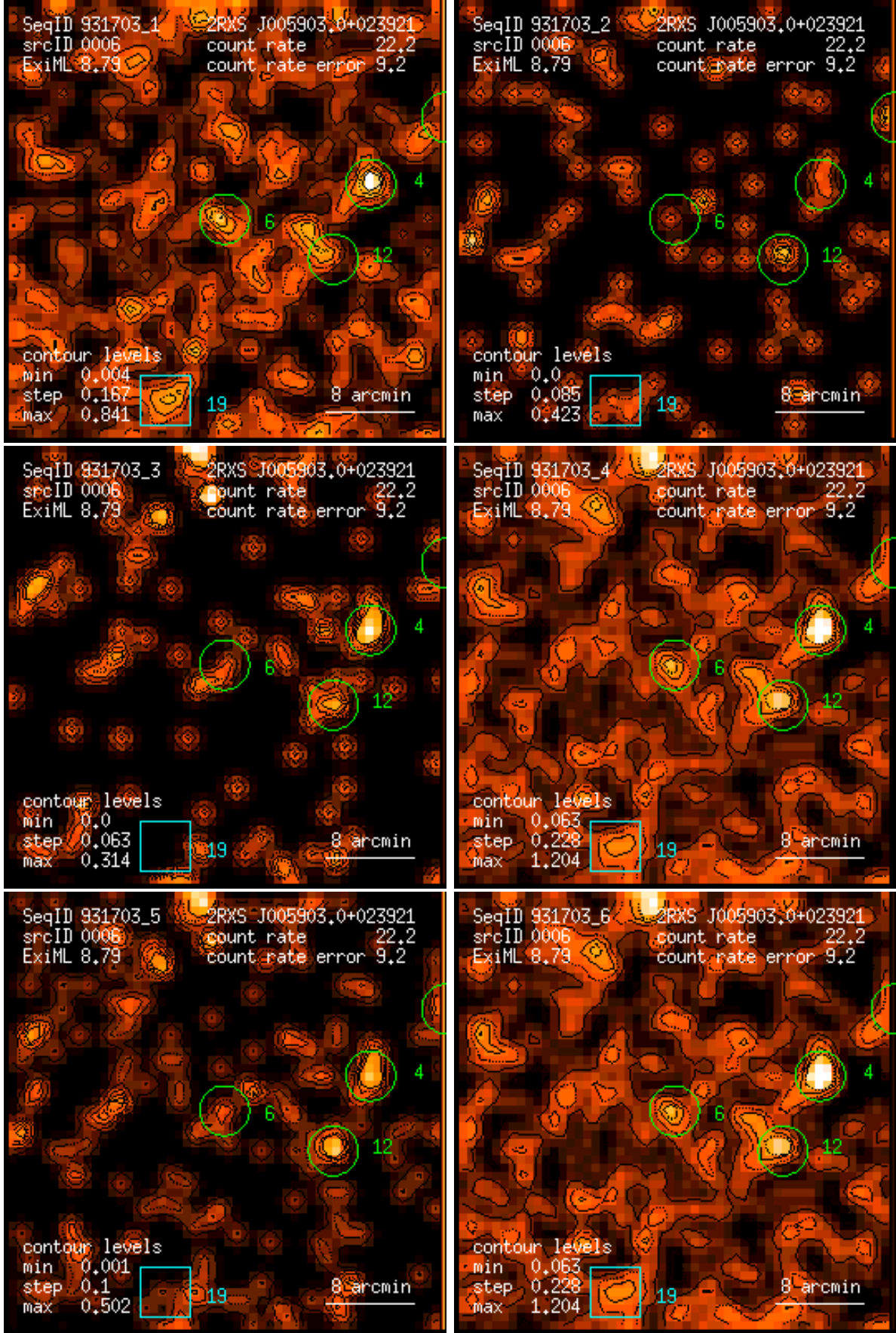
Figure 6: RASS 931703: detection 0006: band rate images, Gaussian filter: (1) PSPC channels 11 – 41, (2) 52 – 90, (3) 91 – 201, (4) 11 – 235, (5) 52 – 201, (6) 11 – 201. Broad band rates in counts/ks. Band rate contour levels in counts/ks/arcmin 2 .
