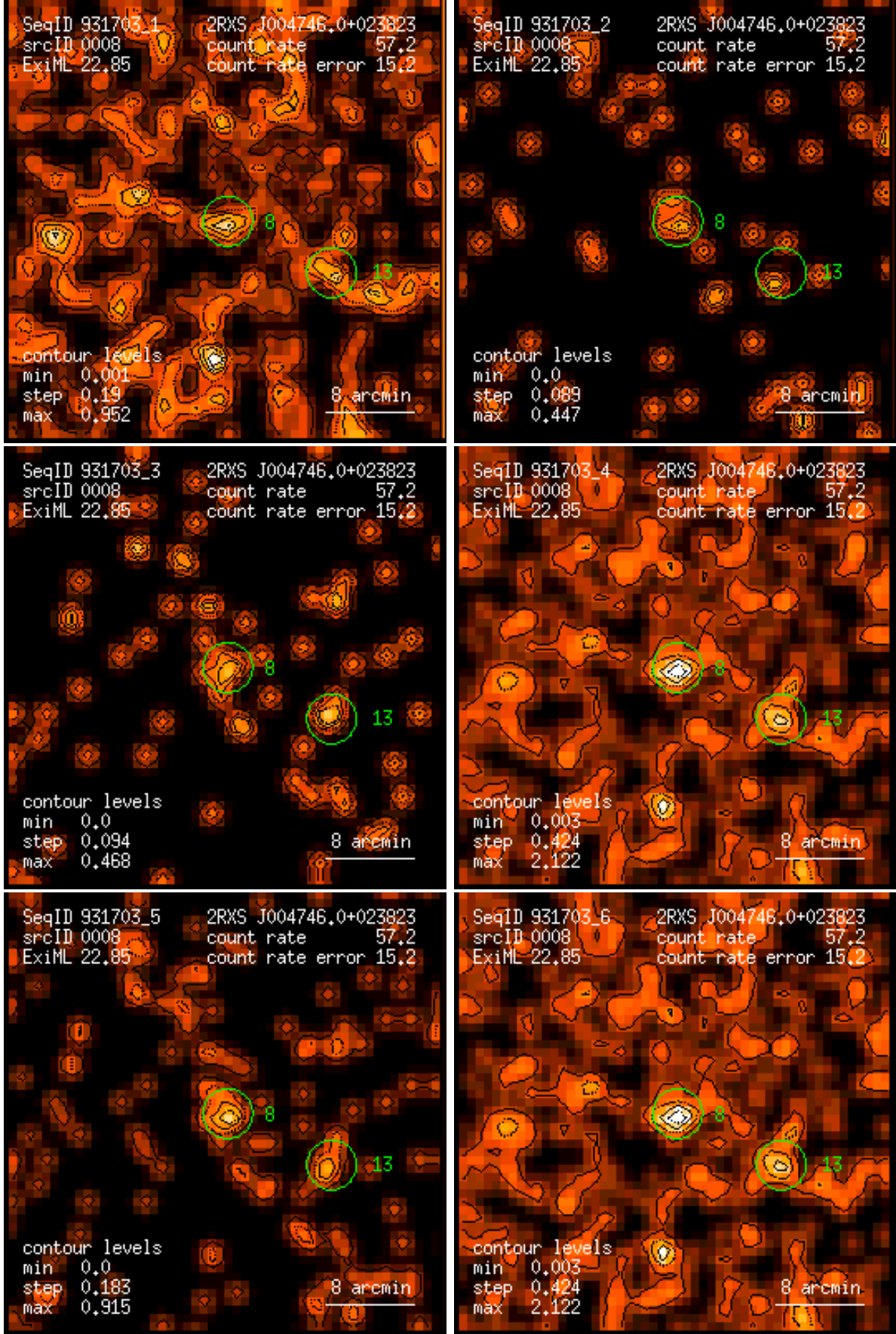
Figure 8: RASS 931703: detection 0008: band rate images, Gaussian filter: (1) PSPC channels 11 – 41, (2) 52 – 90, (3) 91 – 201, (4) 11 – 235, (5) 52 – 201, (6) 11 – 201. Broad band rates in counts/ks. Band rate contour levels in counts/ks/arcmin 2 .
