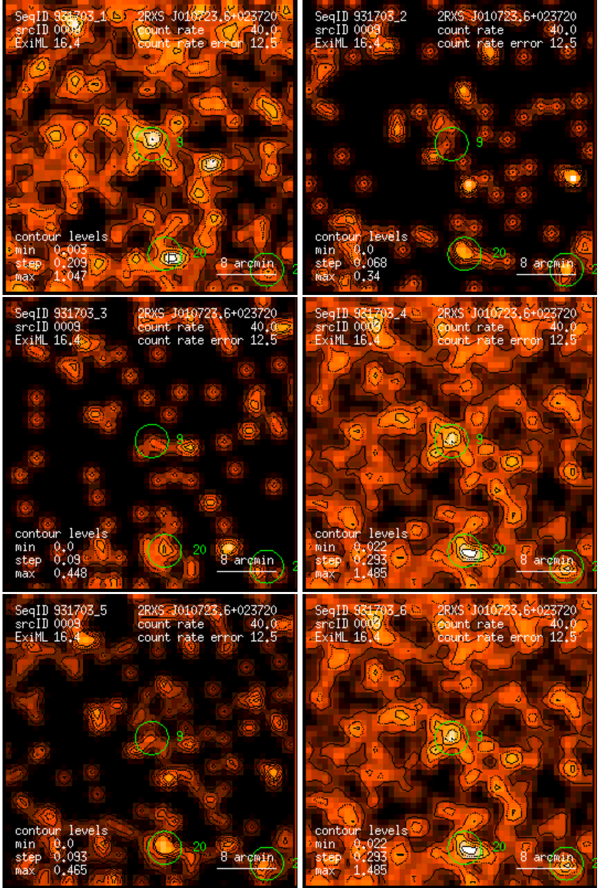
Figure 9: RASS 931703: detection 0009: band rate images, Gaussian filter: (1) PSPC channels 11 – 41, (2) 52 – 90, (3) 91 – 201, (4) 11 – 235, (5) 52 – 201, (6) 11 – 201. Broad band rates in counts/ks. Band rate contour levels in counts/ks/arcmin 2 .
