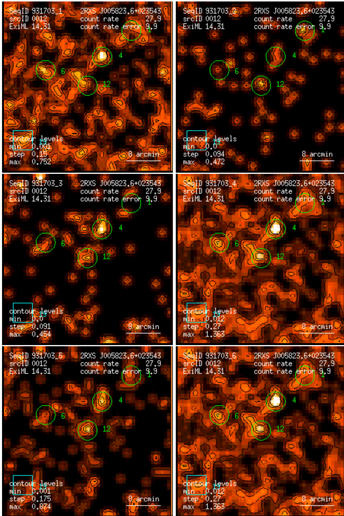
Figure 12: RASS 931703: detection 0012: band rate images, Gaussian filter: (1) PSPC channels 11 – 41, (2) 52 – 90, (3) 91 – 201, (4) 11 – 235, (5) 52 – 201, (6) 11 – 201. Broad band rates in counts/ks. Band rate contour levels in counts/ks/arcmin 2 .
