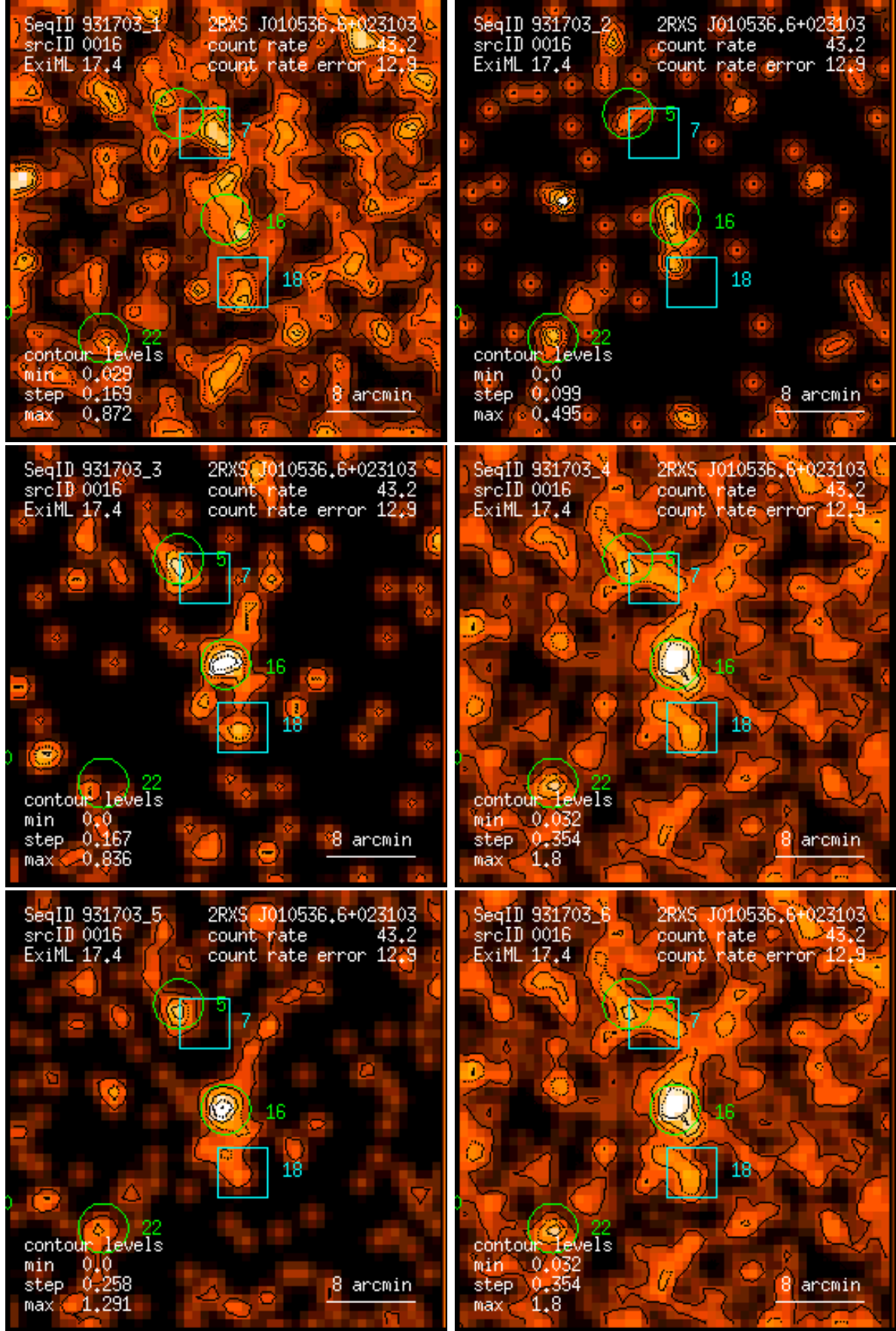
Figure 16: RASS 931703: detection 0016: band rate images, Gaussian filter: (1) PSPC channels 11 – 41, (2) 52 – 90, (3) 91 – 201, (4) 11 – 235, (5) 52 – 201, (6) 11 – 201. Broad band rates in counts/ks. Band rate contour levels in counts/ks/arcmin 2 .
