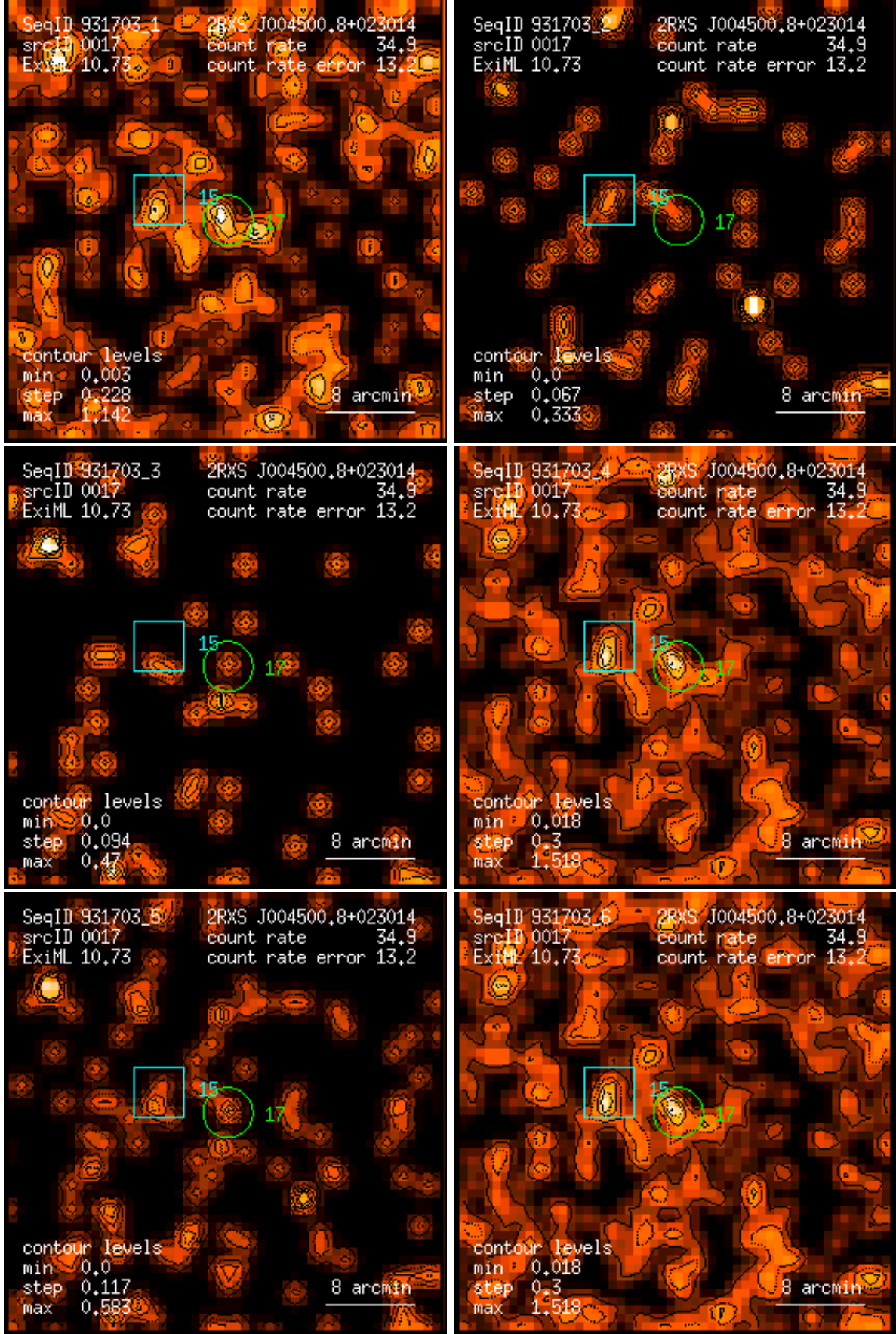
Figure 17: RASS 931703: detection 0017: band rate images, Gaussian filter: (1) PSPC channels 11 – 41, (2) 52 – 90, (3) 91 – 201, (4) 11 – 235, (5) 52 – 201, (6) 11 – 201. Broad band rates in counts/ks. Band rate contour levels in counts/ks/arcmin 2 .
