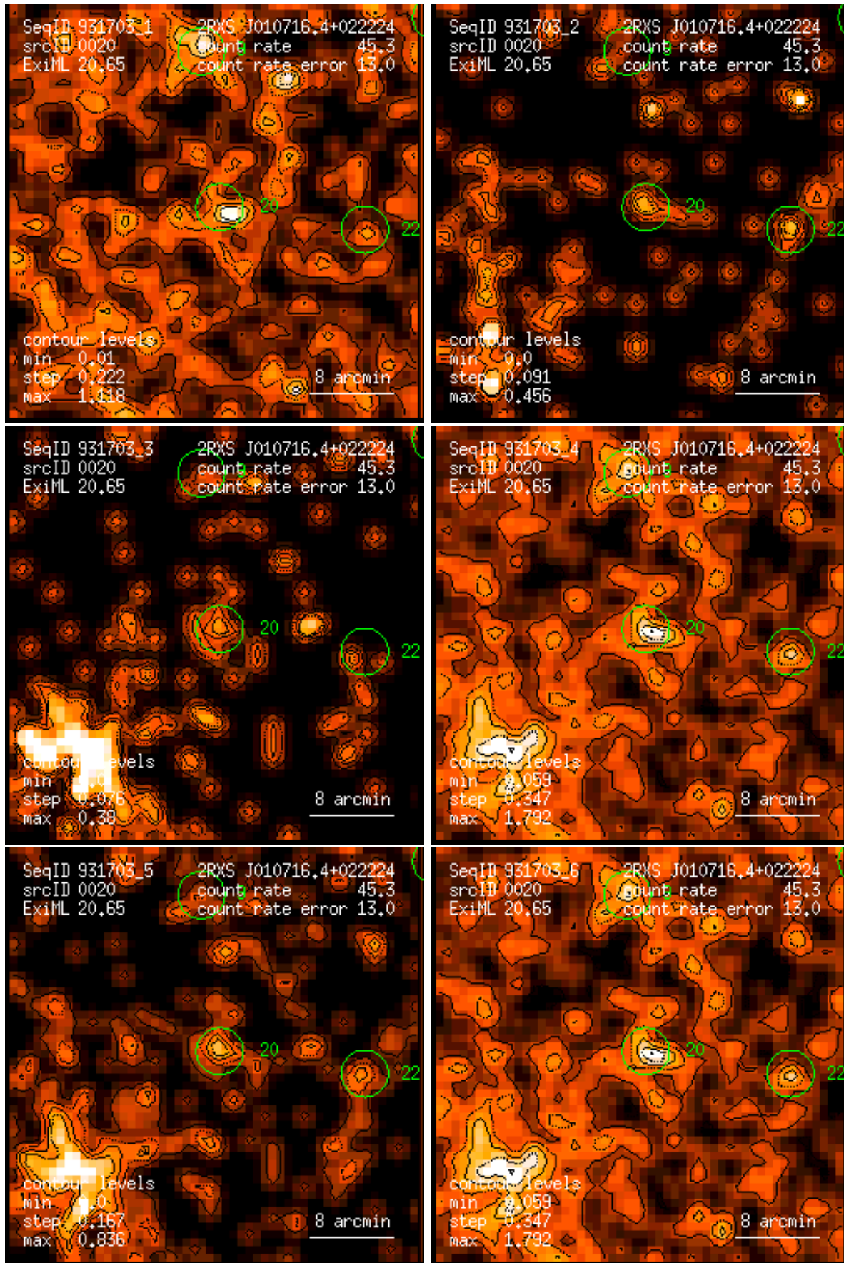
Figure 20: RASS 931703: detection 0020: band rate images, Gaussian filter: (1) PSPC channels 11 – 41, (2) 52 – 90, (3) 91 – 201, (4) 11 – 235, (5) 52 – 201, (6) 11 – 201. Broad band rates in counts/ks. Band rate contour levels in counts/ks/arcmin 2 .
