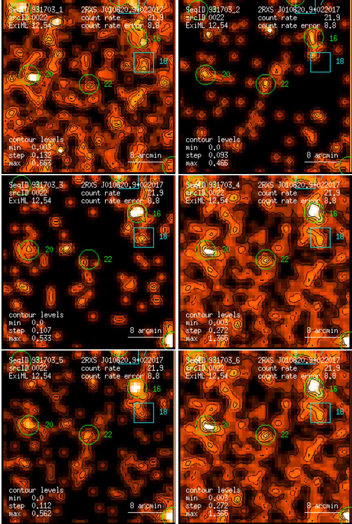
Figure 22: RASS 931703: detection 0022: band rate images, Gaussian filter: (1) PSPC channels 11 – 41, (2) 52 – 90, (3) 91 – 201, (4) 11 – 235, (5) 52 – 201, (6) 11 – 201. Broad band rates in counts/ks. Band rate contour levels in counts/ks/arcmin 2 .
