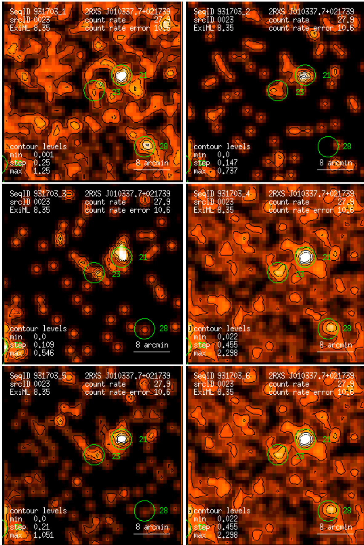
Figure 23: RASS 931703: detection 0023: band rate images, Gaussian filter: (1) PSPC channels 11 – 41, (2) 52 – 90, (3) 91 – 201, (4) 11 – 235, (5) 52 – 201, (6) 11 – 201. Broad band rates in counts/ks. Band rate contour levels in counts/ks/arcmin 2 .
