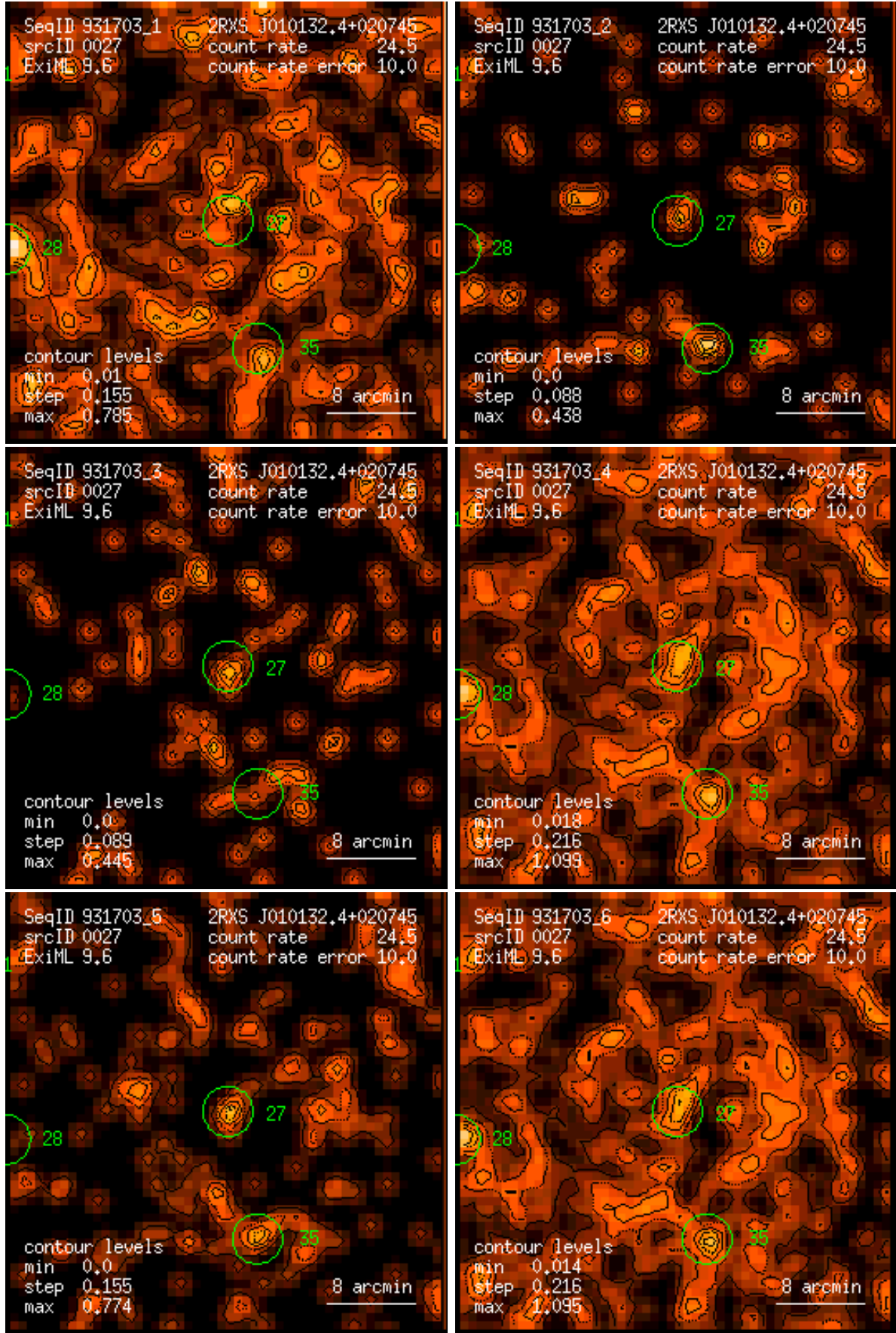
Figure 27: RASS 931703: detection 0027: band rate images, Gaussian filter: (1) PSPC channels 11 – 41, (2) 52 – 90, (3) 91 – 201, (4) 11 – 235, (5) 52 – 201, (6) 11 – 201. Broad band rates in counts/ks. Band rate contour levels in counts/ks/arcmin 2 .
